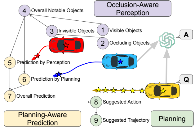
Fig. 1: Illustration of our proposed graph-of-thoughts reasoning framework for cooperative autonomous driving.
