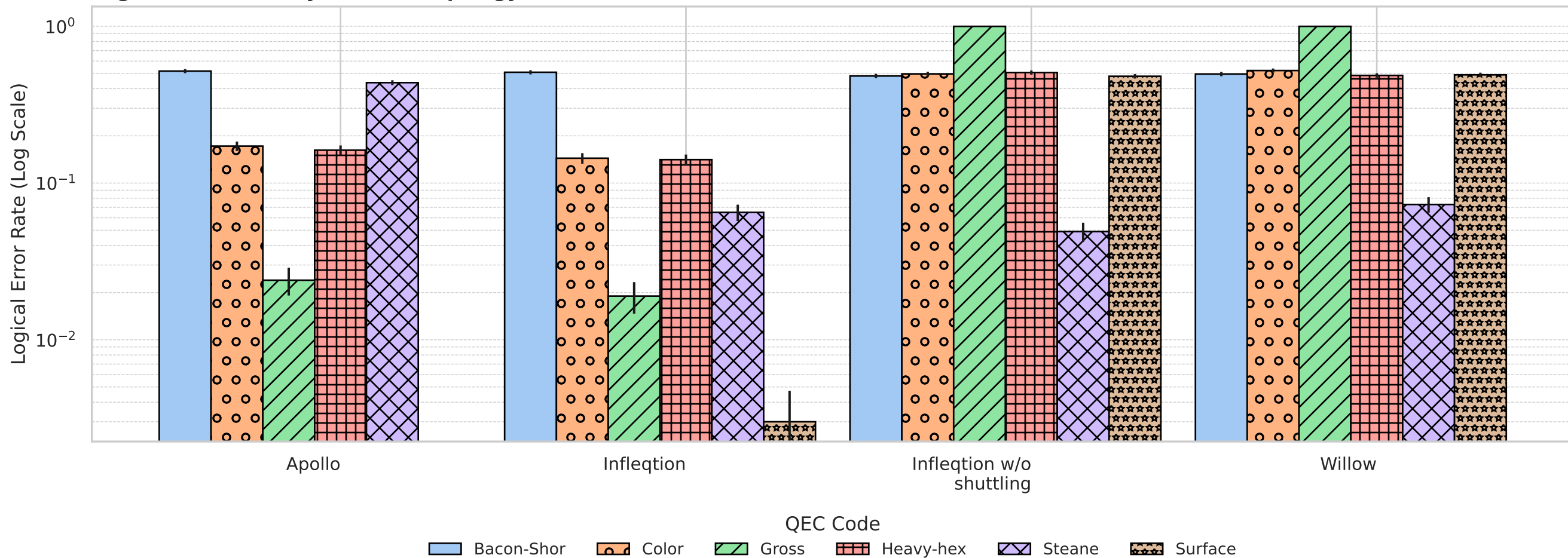
Logical Error Rate by Backend Topology
