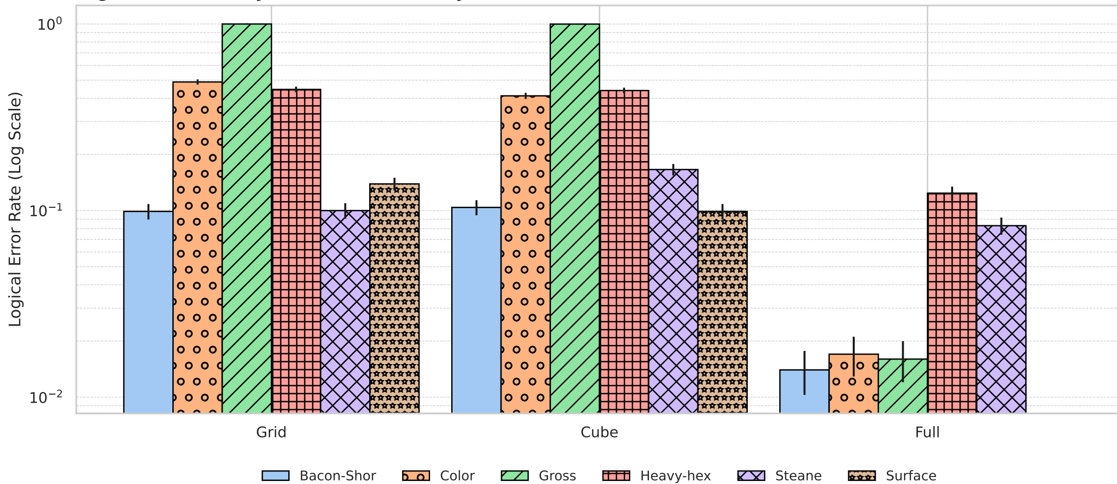
Logical Error Rate by Backend Connectivity
