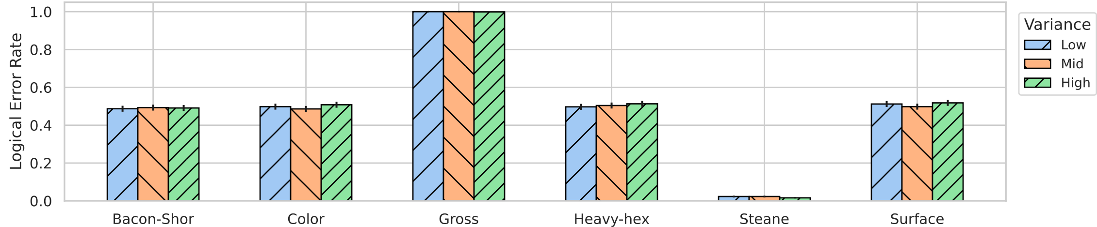
Logical Error Rate by Code (with Std Dev)
