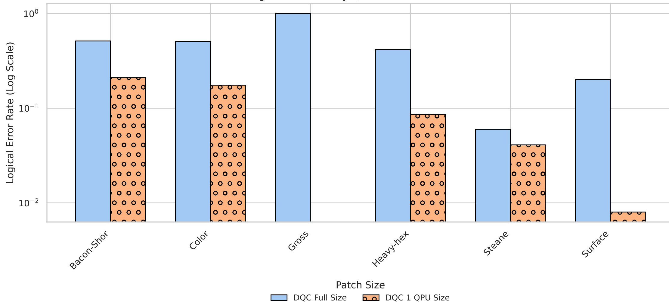
Logical Error Rate by QEC Code and Patch Size
