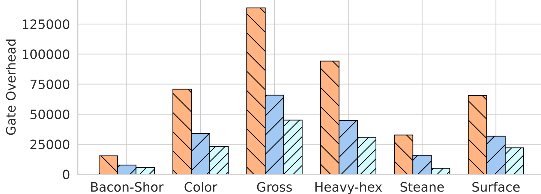
(a) Gate Overhead (IBM Heron)
