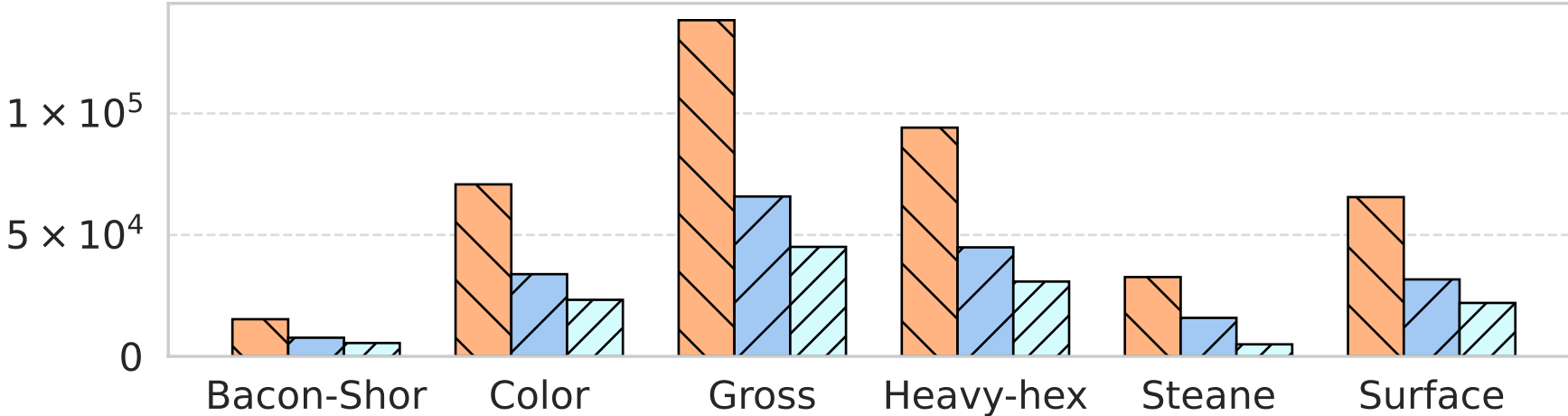
(a) Gate Overhead (IBM Heron)
