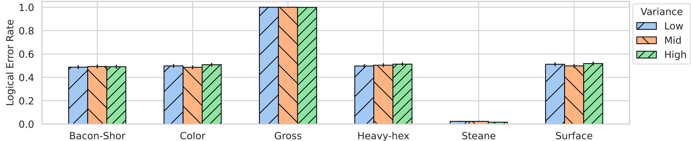
Logical Error Rate by Code (with Std Dev)
