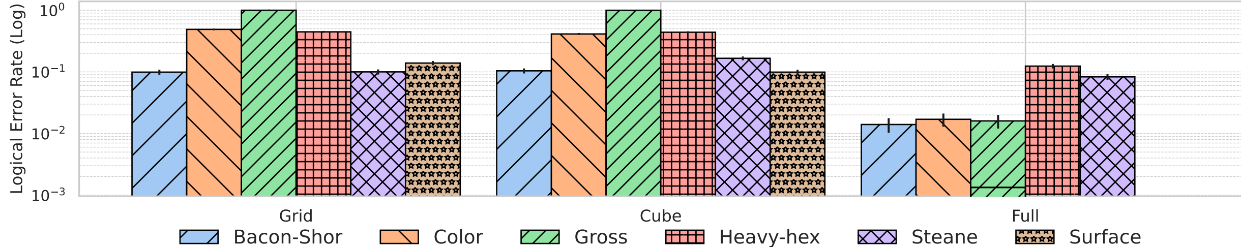
Logical Error Rate by Backend Connectivity
