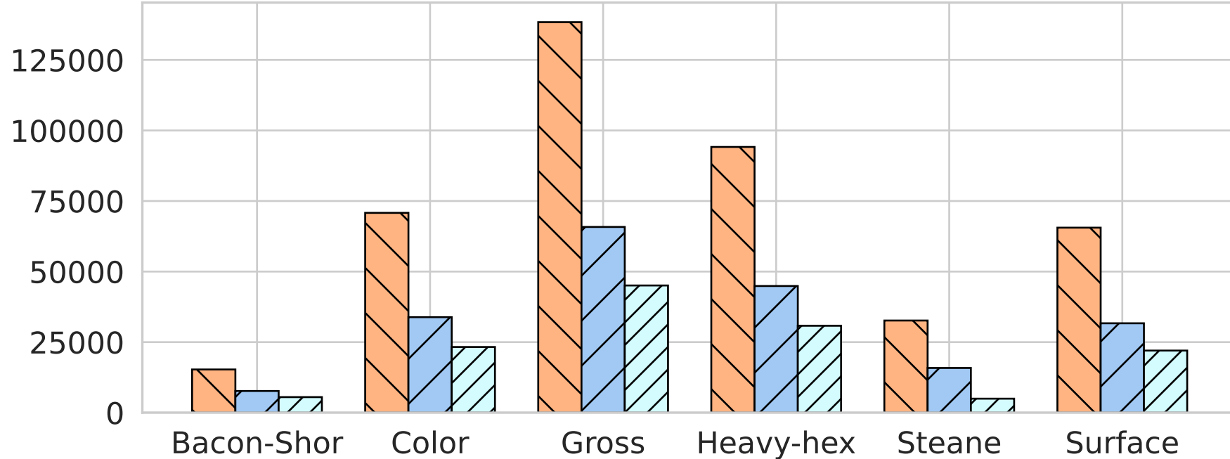
(a) Gate Overhead (IBM Heron)
