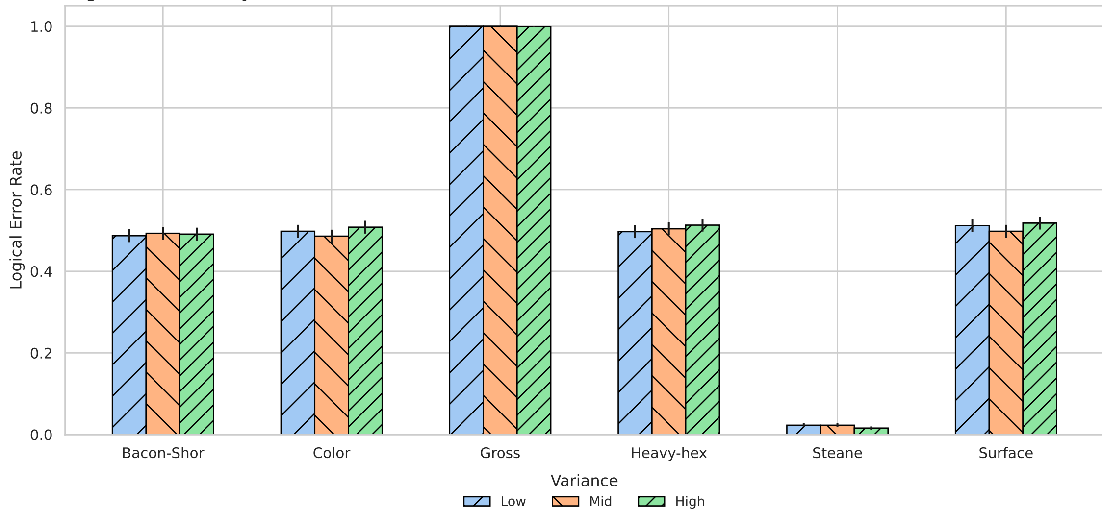
Logical Error Rate by Code (with Std Dev)
