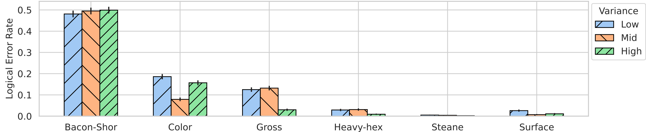
Logical Error Rate by Code
