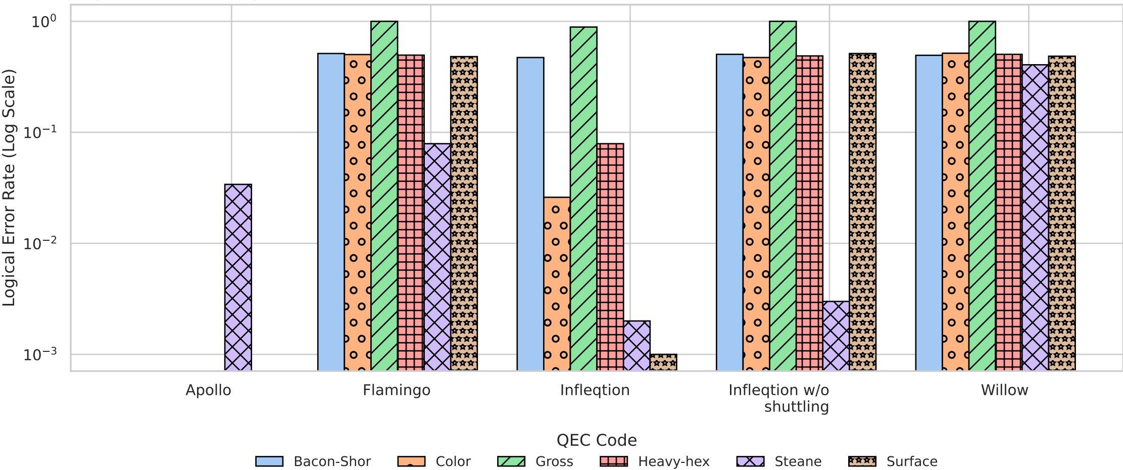
Logical Error Rate by Backend and QEC Code
