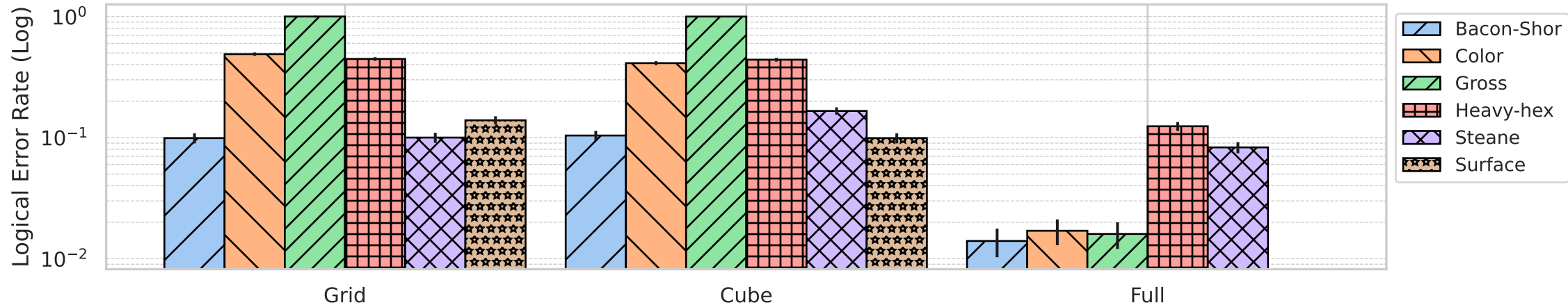
Logical Error Rate by Backend Connectivity
