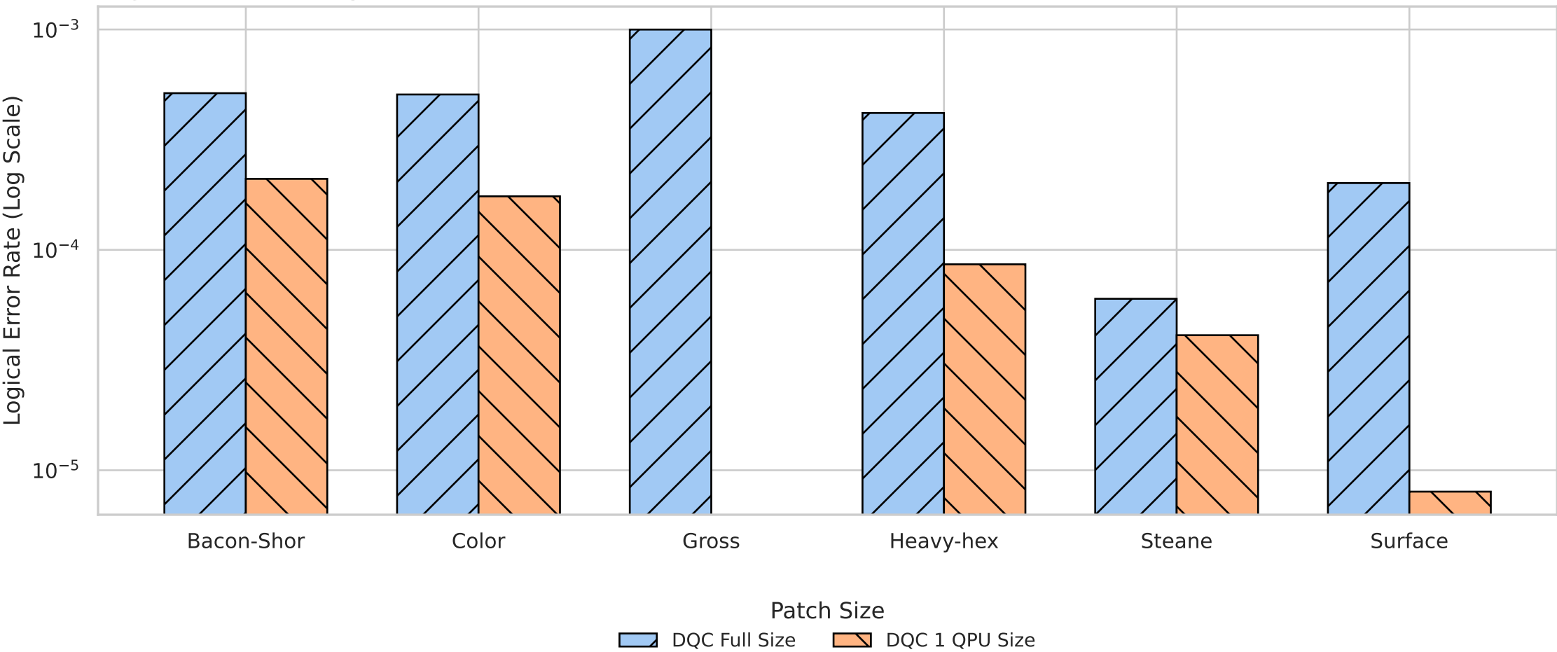
Logical Error Rate by QEC Code and Patch Size
