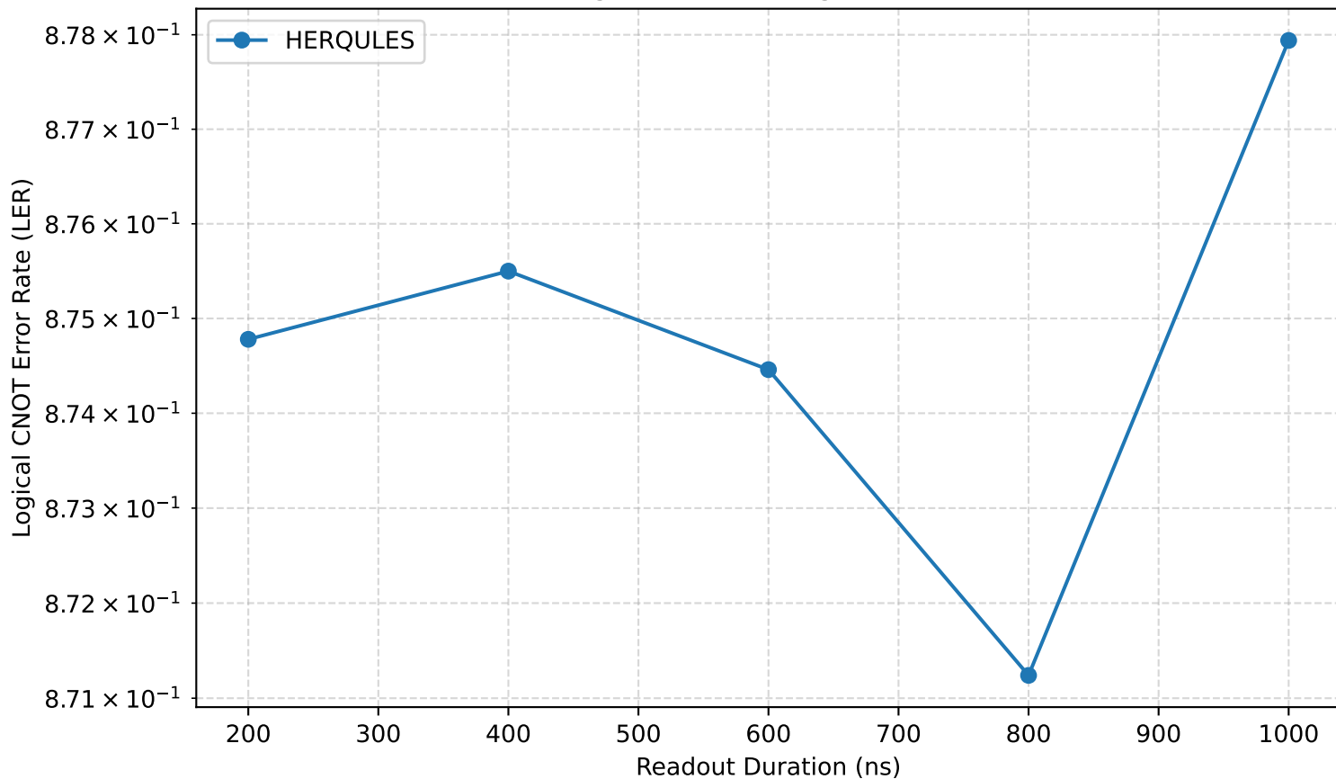
MCM Readout Length vs LER — logical CNOT d=9 (futuristic)
