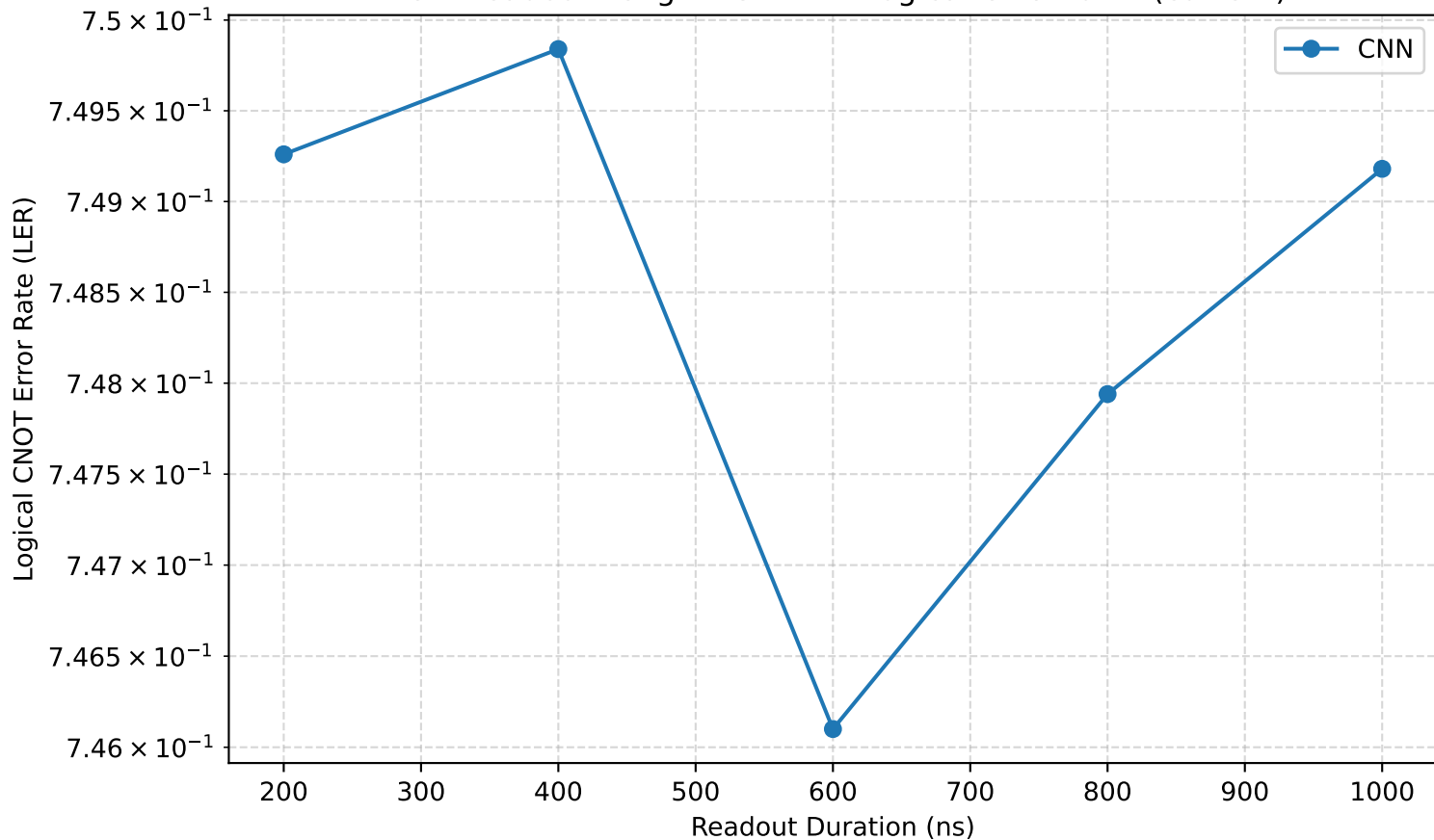
MCM Readout Length vs LER — logical CNOT d=7 (current)
