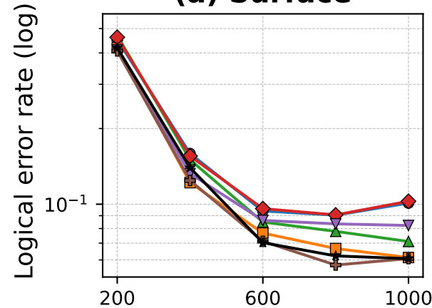
(a) Surface
