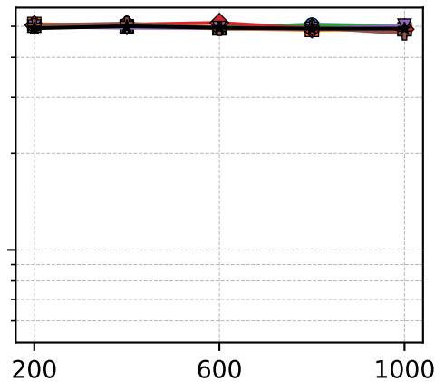
(b) Bacon-shor
