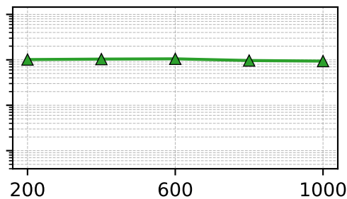
(f) Steane
