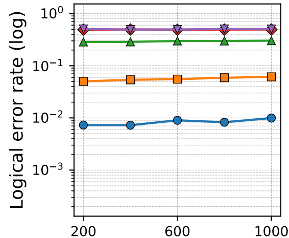
(a) Surface
