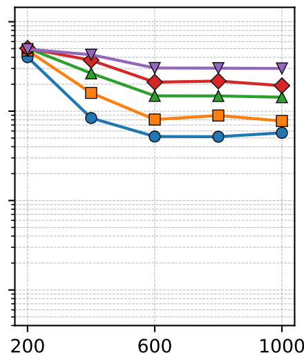
(b) Bacon-shor
