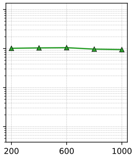
(f) Steane
