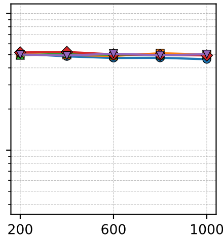
(b) Bacon-shor
