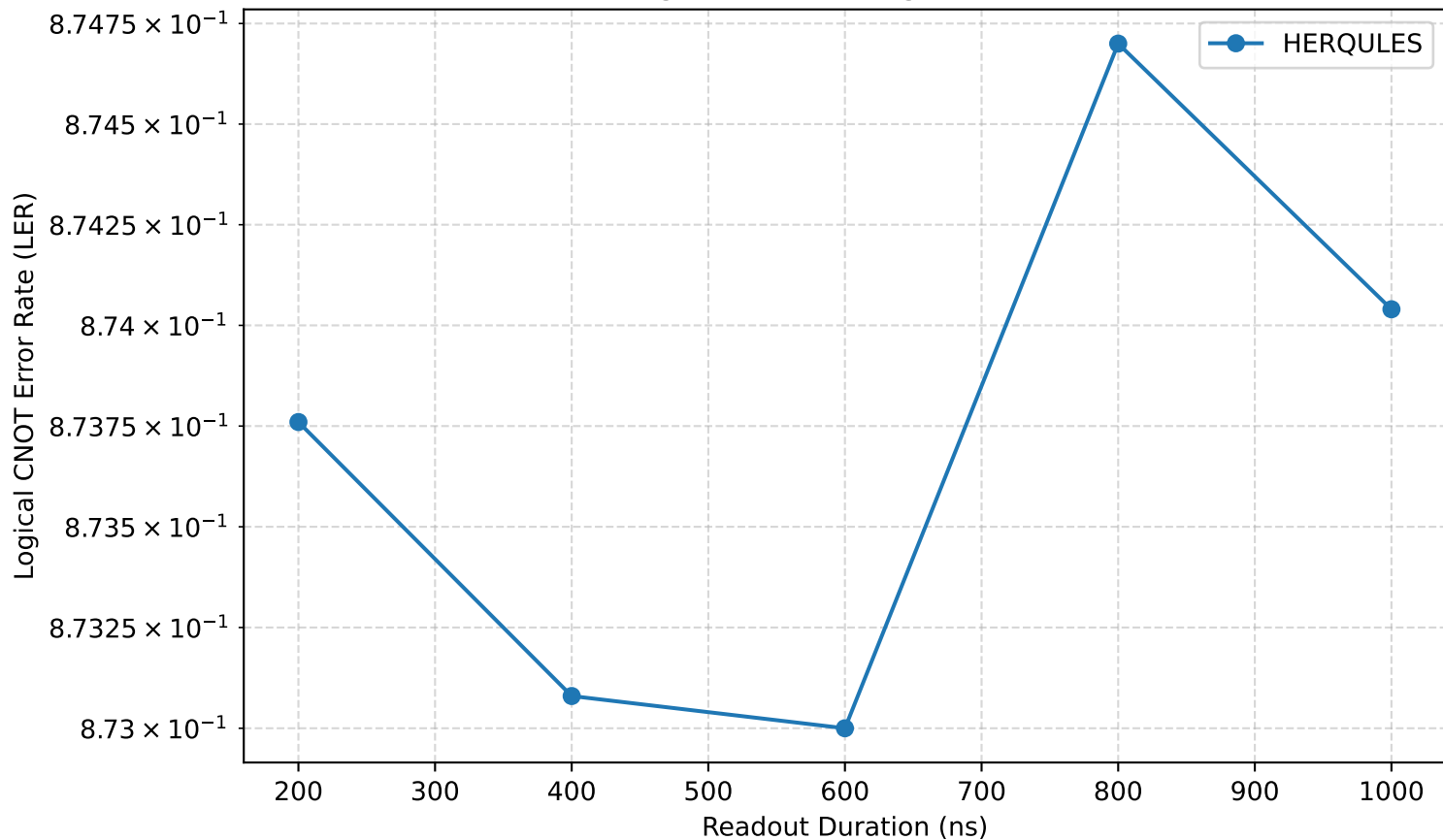
MCM Readout Length vs LER — logical CNOT d=11 (current)
