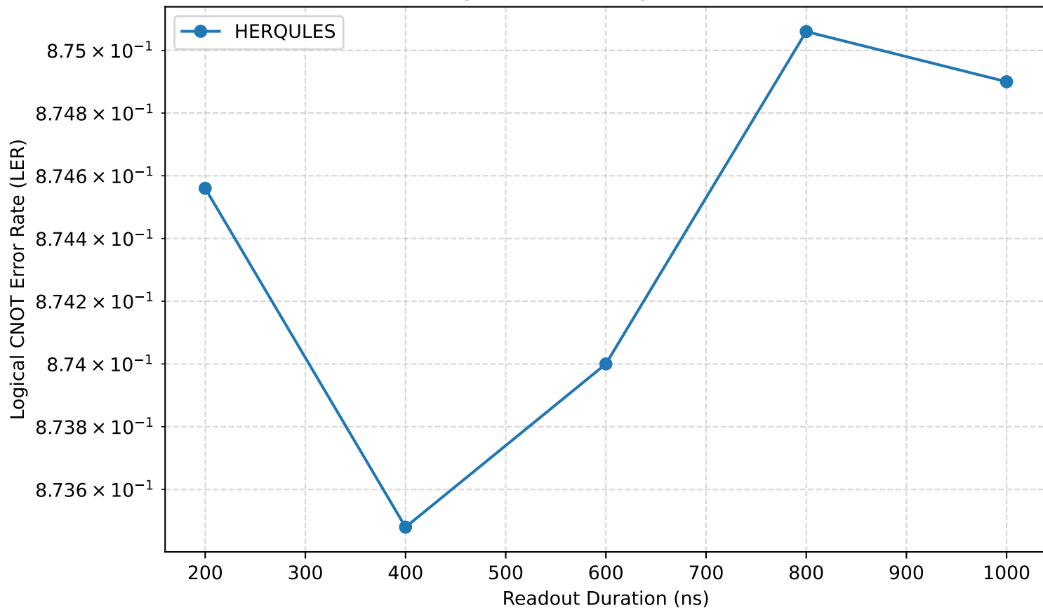
MCM Readout Length vs LER — logical CNOT d=11 (futuristic)
