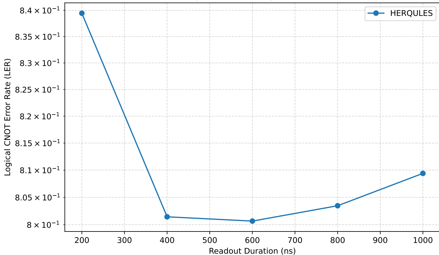
MCM Readout Length vs LER — logical CNOT d=7 (futuristic)
