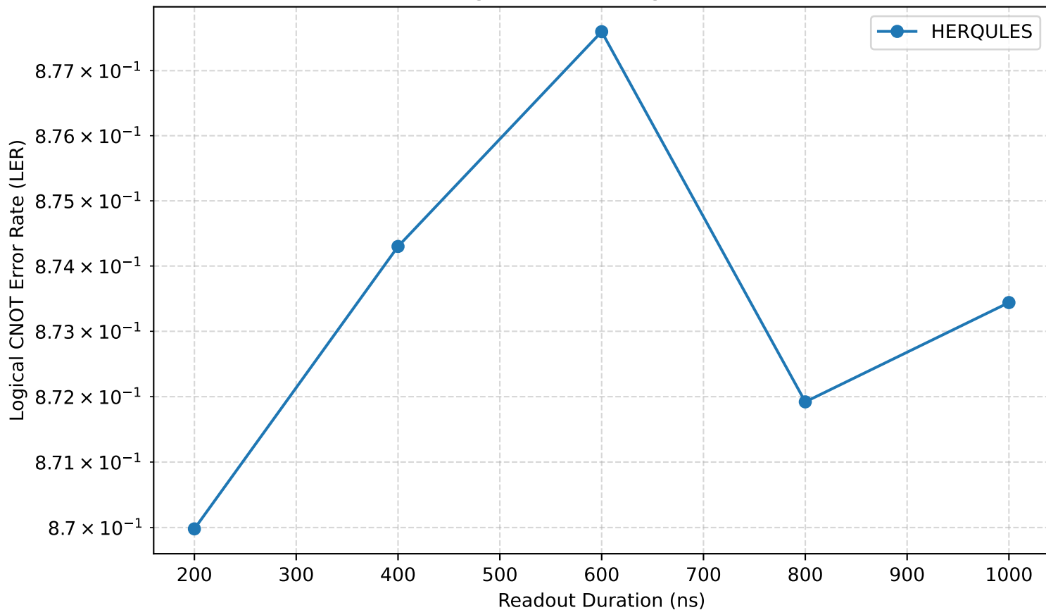
MCM Readout Length vs LER — logical CNOT d=9 (current)
