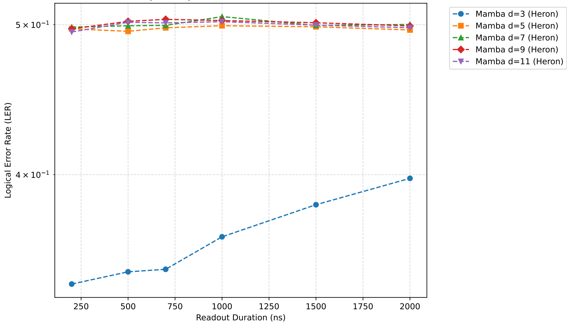
MCM Latency-Fidelity Tradeoff: Color Code (Decode: 10000ns)
