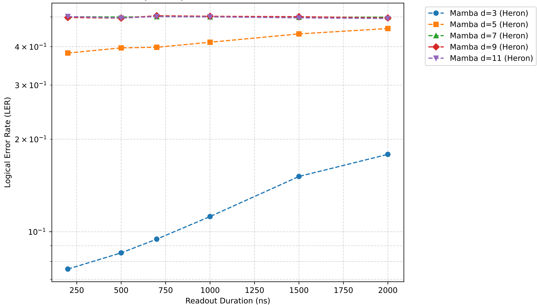
MCM Latency-Fidelity Tradeoff: Color Code (Decode: 1000ns)
