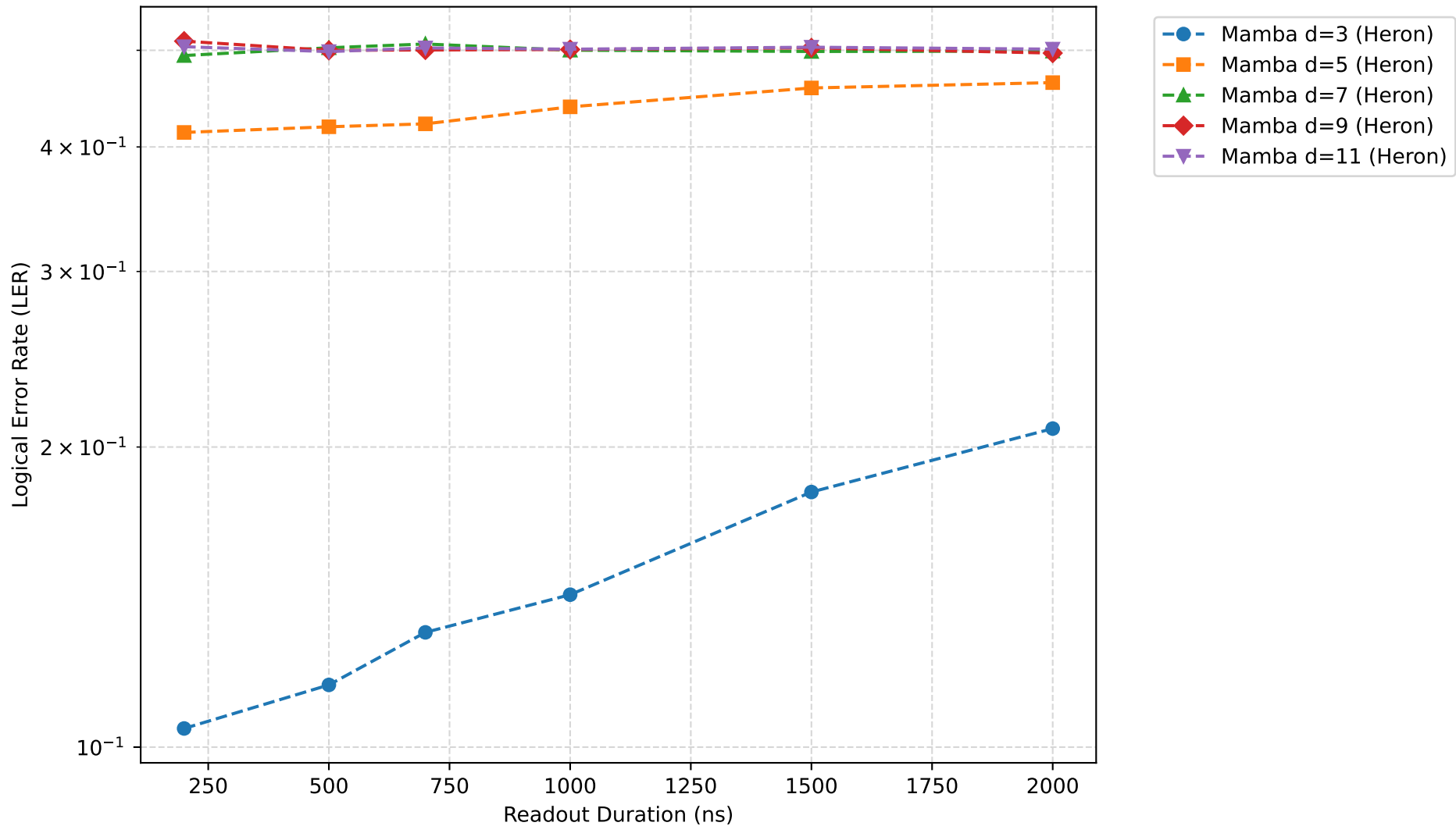
MCM Latency-Fidelity Tradeoff: Color Code (Decode: 2000ns)
