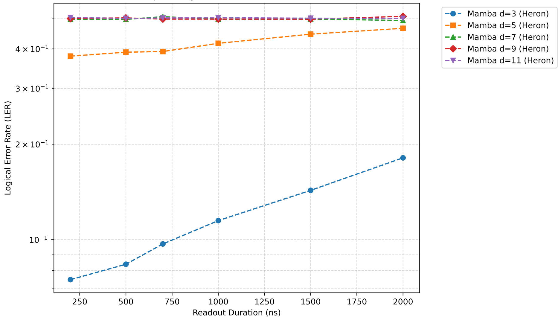
MCM Latency-Fidelity Tradeoff: Color Code (Decode: 500ns)
