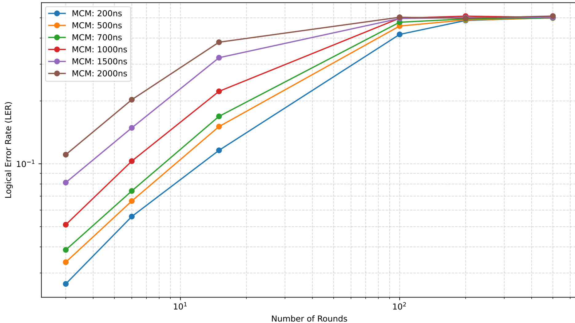
LER vs Rounds (Surface Code d=3, Decode: 500ns)
