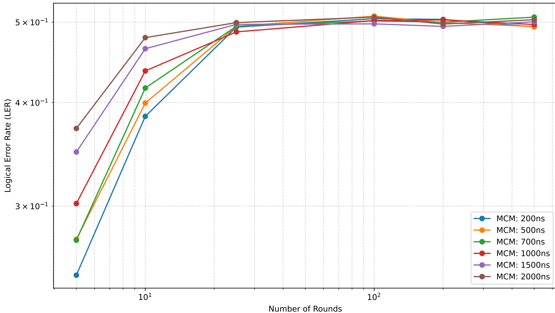
LER vs Rounds (Surface Code d=5, Decode: 500ns)
