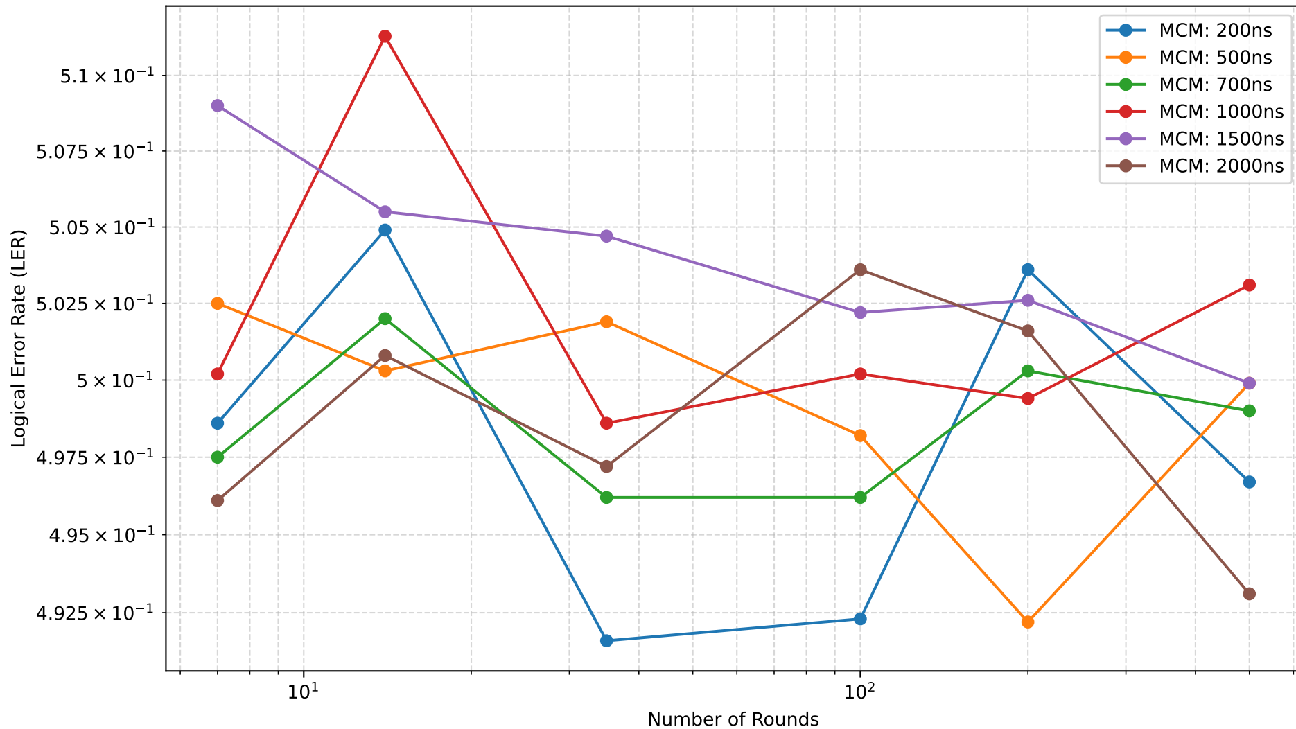
LER vs Rounds (Surface Code d=7, Decode: 500ns)
