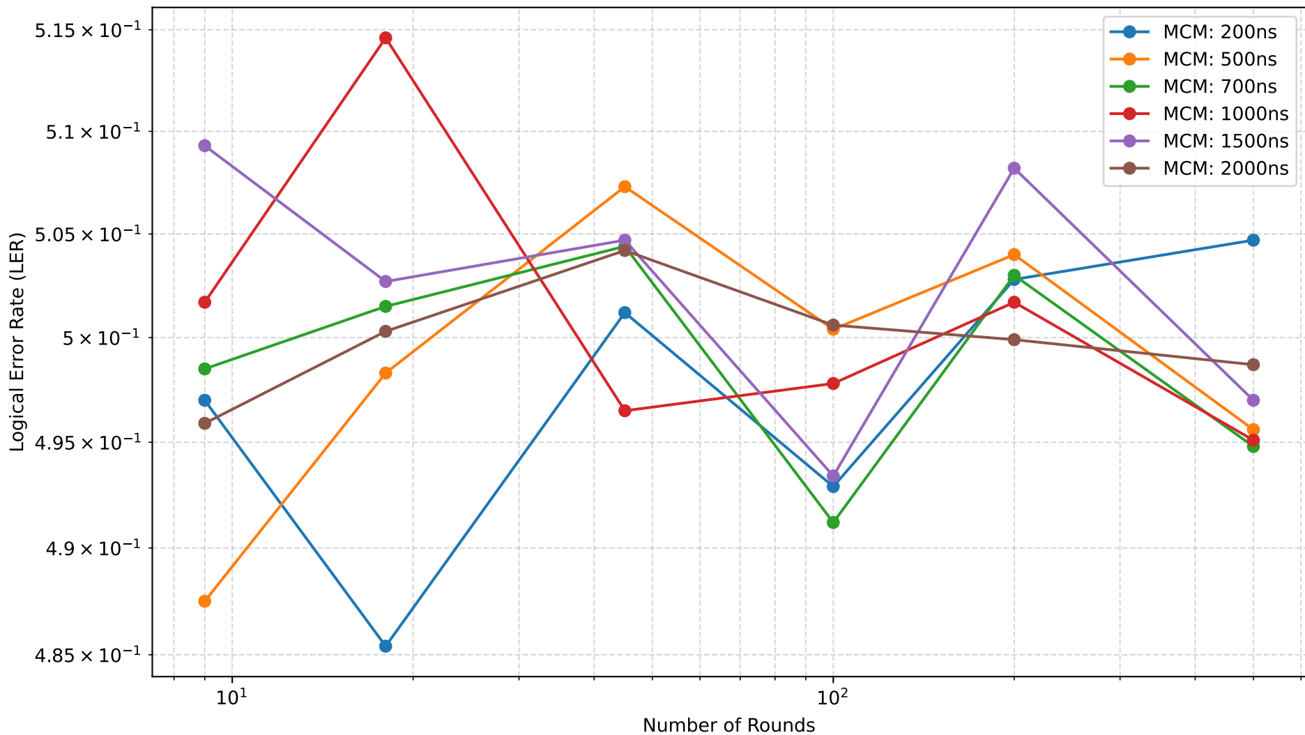
LER vs Rounds (Surface Code d=9, Decode: 500ns)
