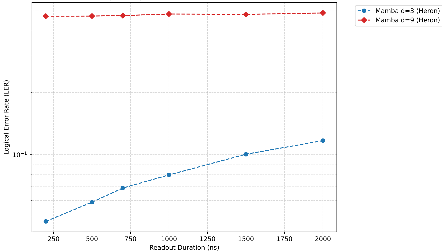
MCM Latency-Fidelity Tradeoff: Steane Code (Decode: 10000ns)
