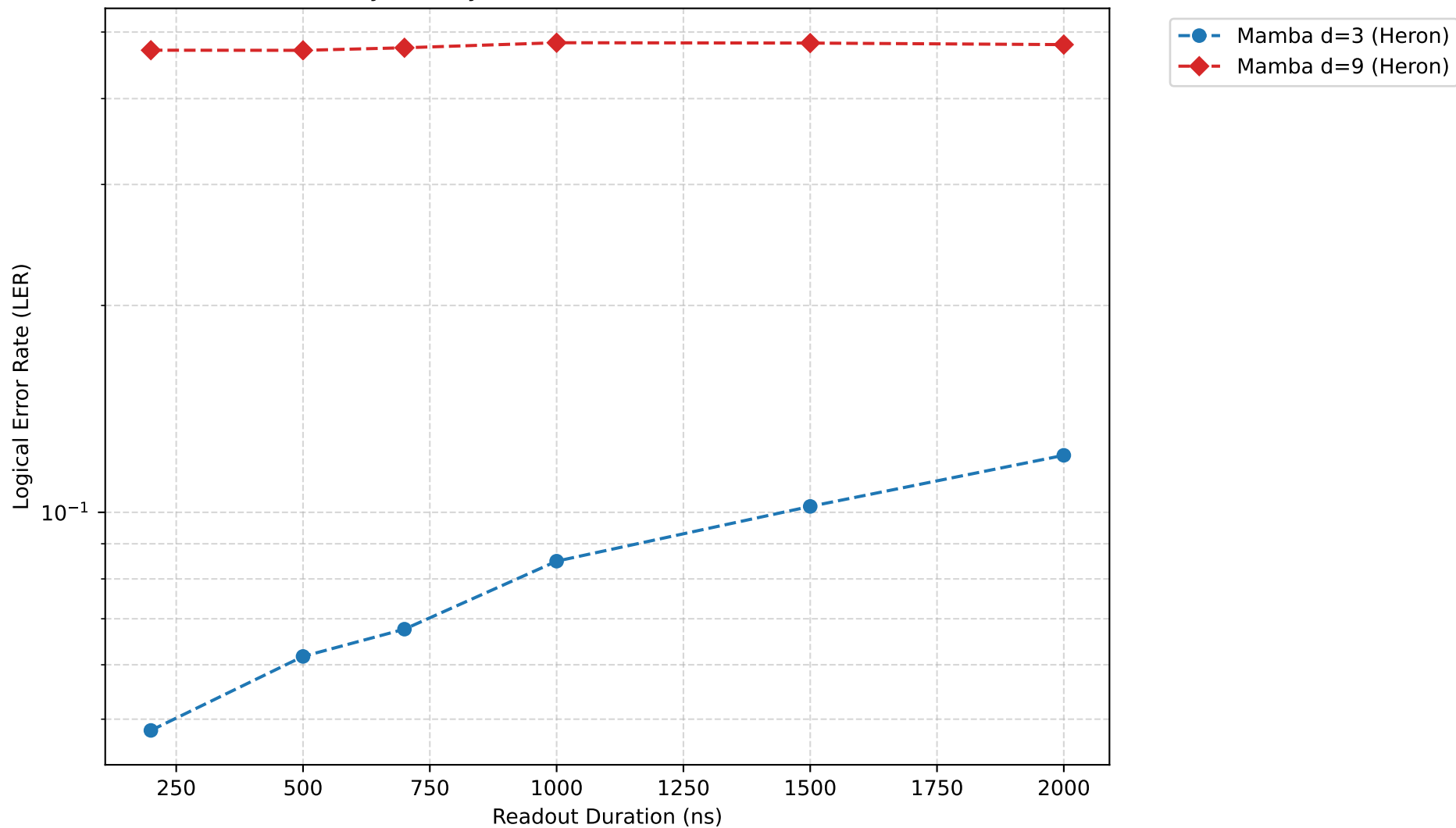
MCM Latency-Fidelity Tradeoff: Steane Code (Decode: 1000ns)
