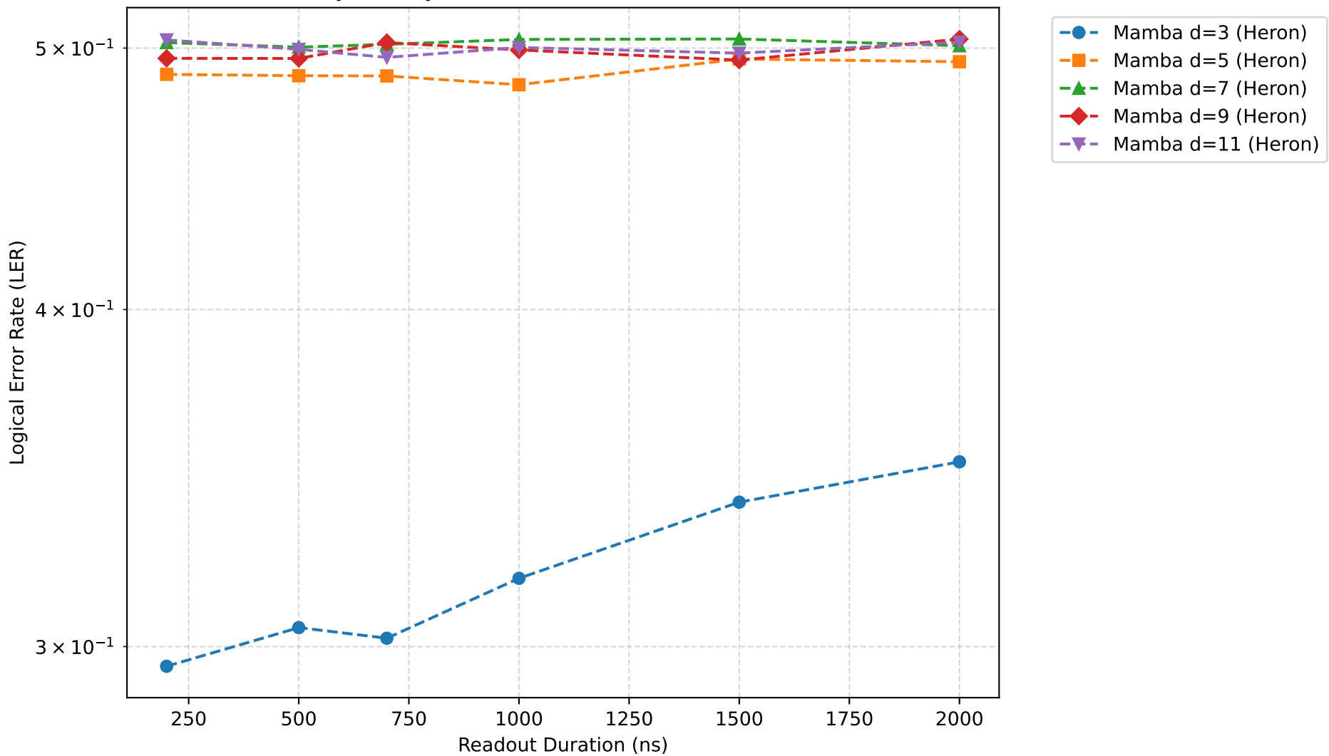
MCM Latency-Fidelity Tradeoff: Surface Code (Decode: 10000ns)
