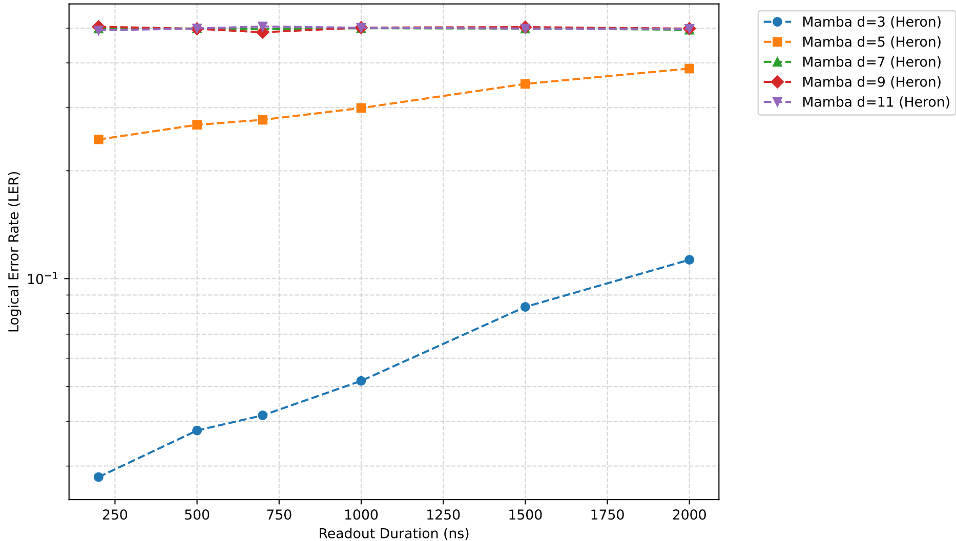
MCM Latency-Fidelity Tradeoff: Surface Code (Decode: 1000ns)
