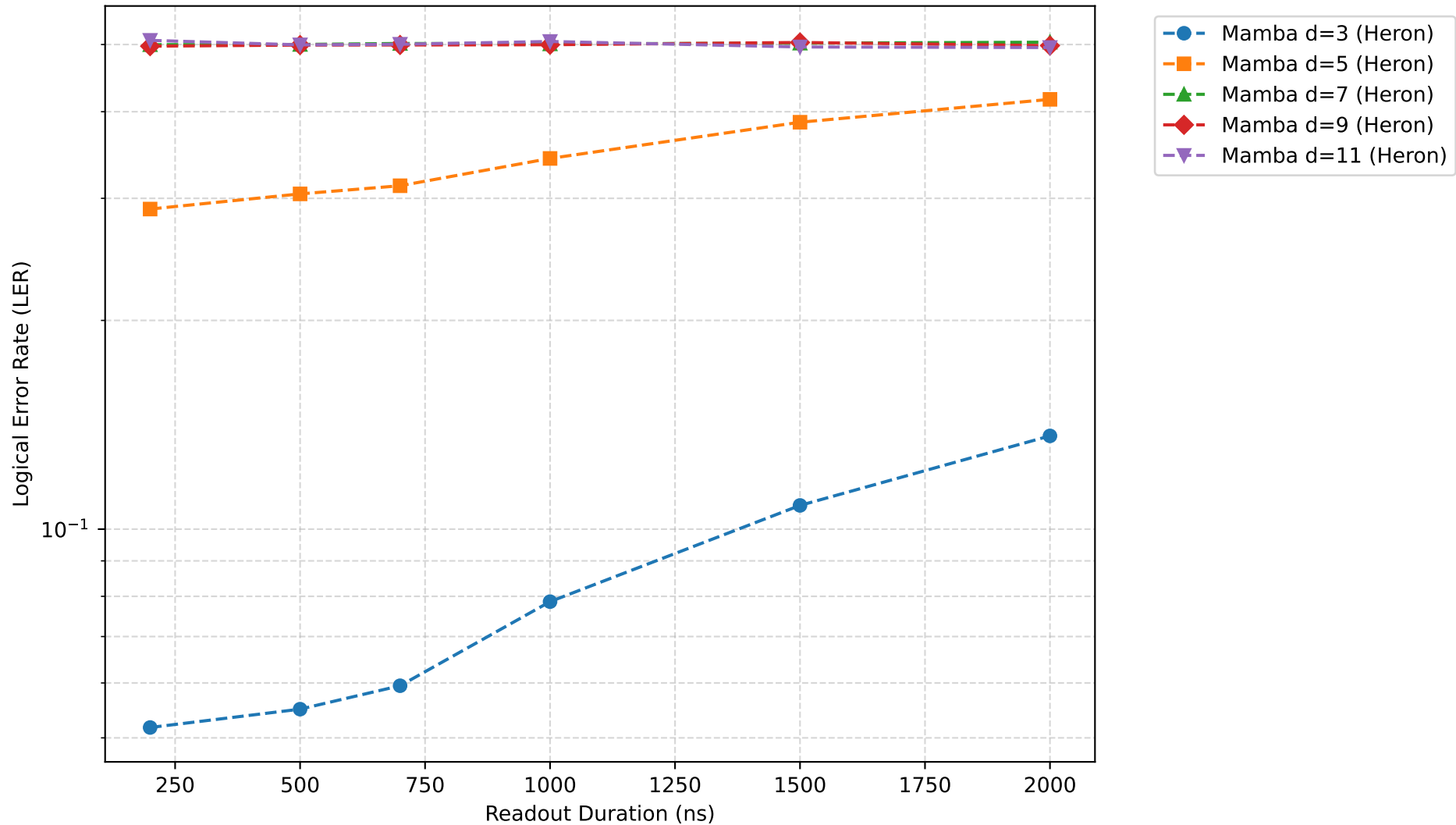
MCM Latency-Fidelity Tradeoff: Surface Code (Decode: 2000ns)
