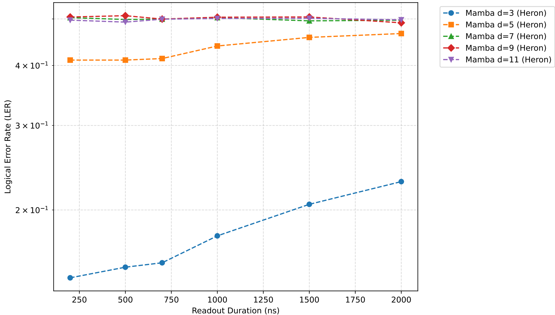
MCM Latency-Fidelity Tradeoff: Surface Code (Decode: 5000ns)
