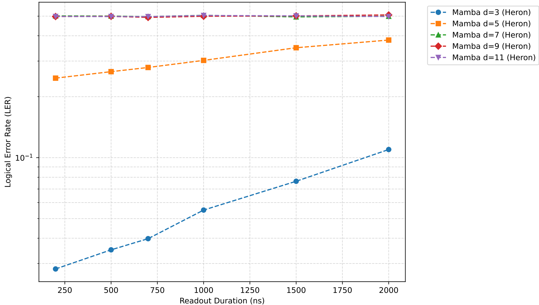
MCM Latency-Fidelity Tradeoff: Surface Code (Decode: 500ns)
