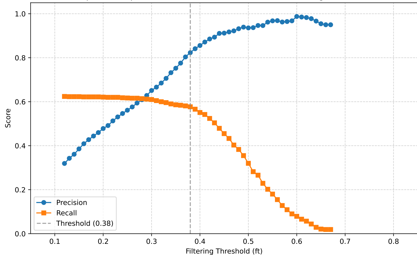
Comparison of precision and recall based on the final filtering threshold (ft)
