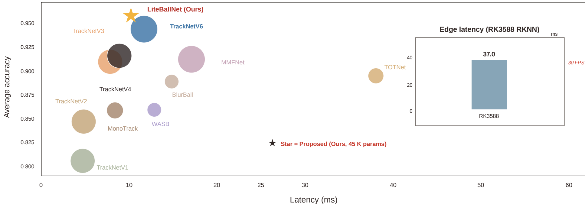
Avg. Acc. vs. Latency (3 Benchmarks)
