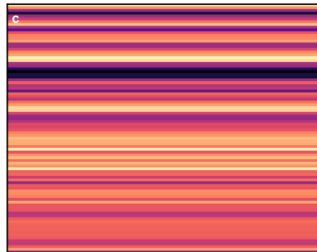
Output heatmap
