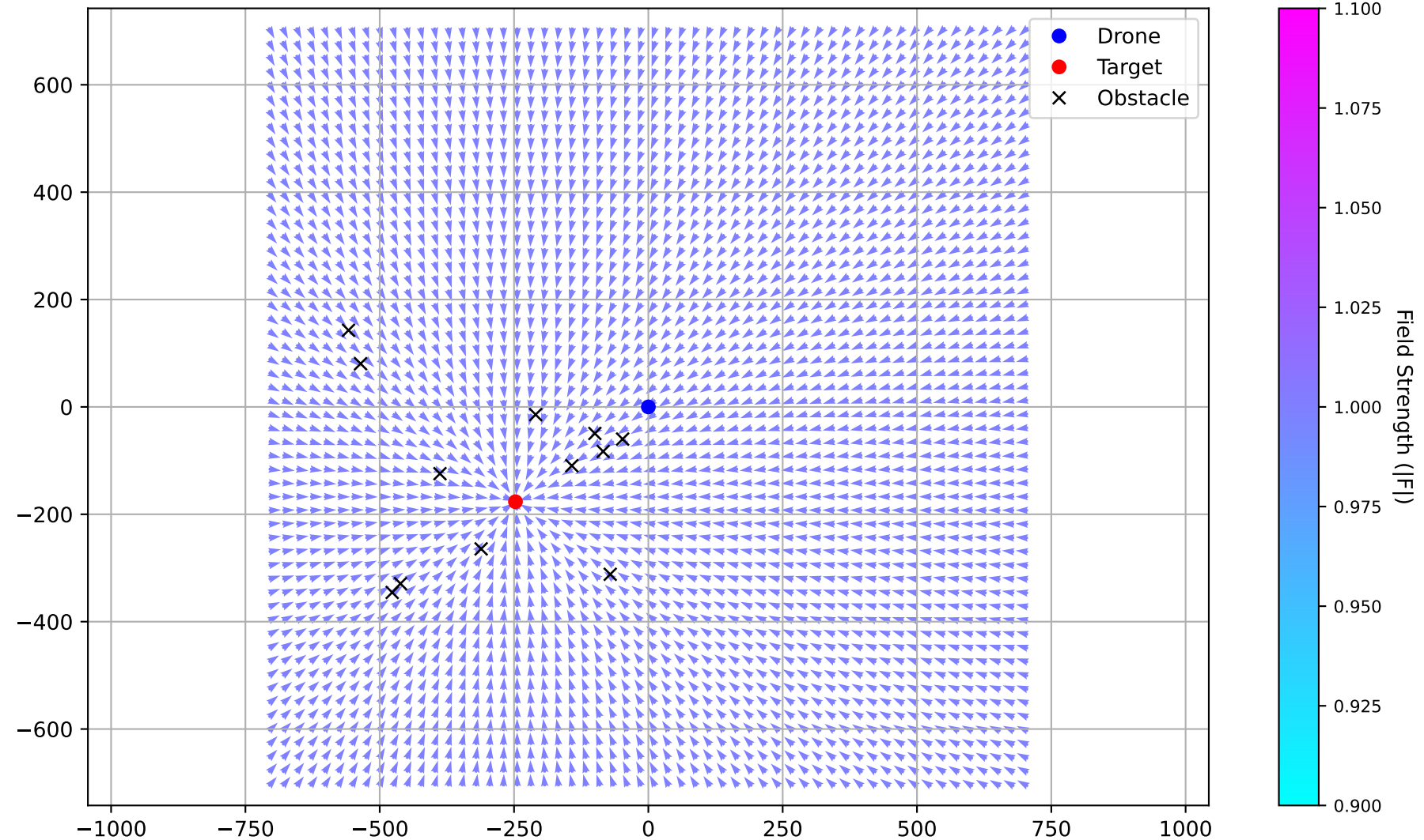
World barrier function (relative to drone)
