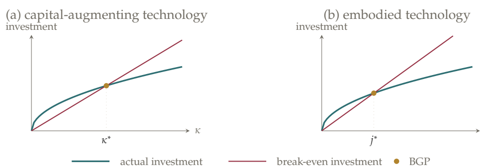
Figure 1.8. Normalized dynamics under capital-augmenting and embodied technological progress. The break-even schedules are (n + \phi\mu + \delta)\kappa and [n + \delta + (1 + \phi)\mu]j , respectively.
