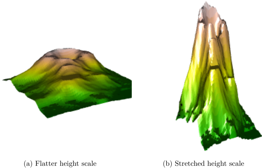
Figure 2.13: Two figures representing the volcano dataset (R Core Team 2024) using different height scaling factors. Both figures use the same color scale, but there is no “correct” translation of color into the measurable height.
