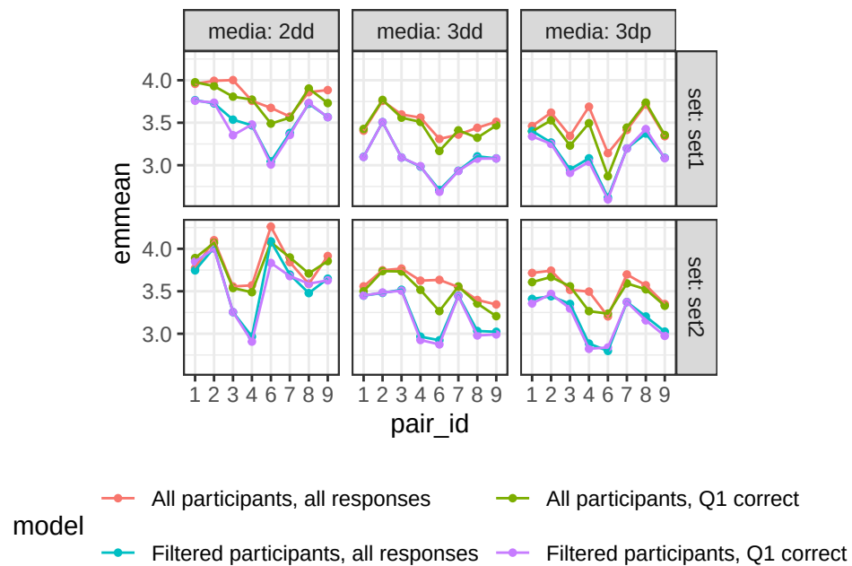
Figure 5.20: Interaction plots for stimuli pairs and response filtering, faceted by dataset and media type.
