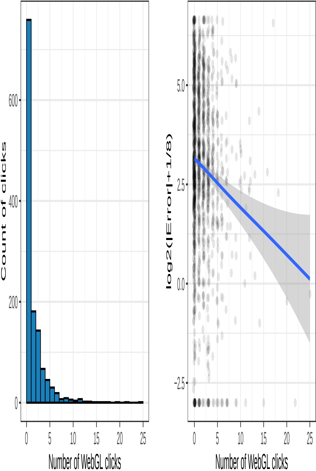
(a) Histogram
