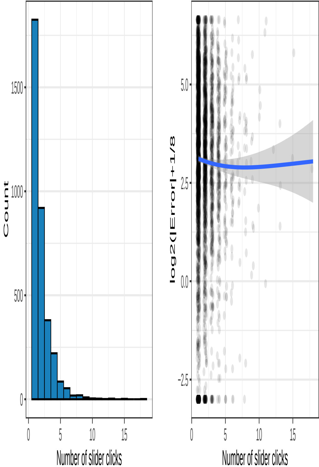
(a) Histogram
