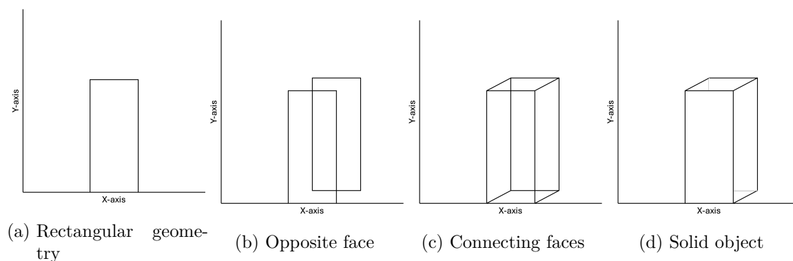
Figure 2.4: Construction of depth cues for a 2D bar chart. First, the amount of depth is set by defining the opposite face of the standard 2D rectangular shape. Then the faces are connected and volume is filled in.
