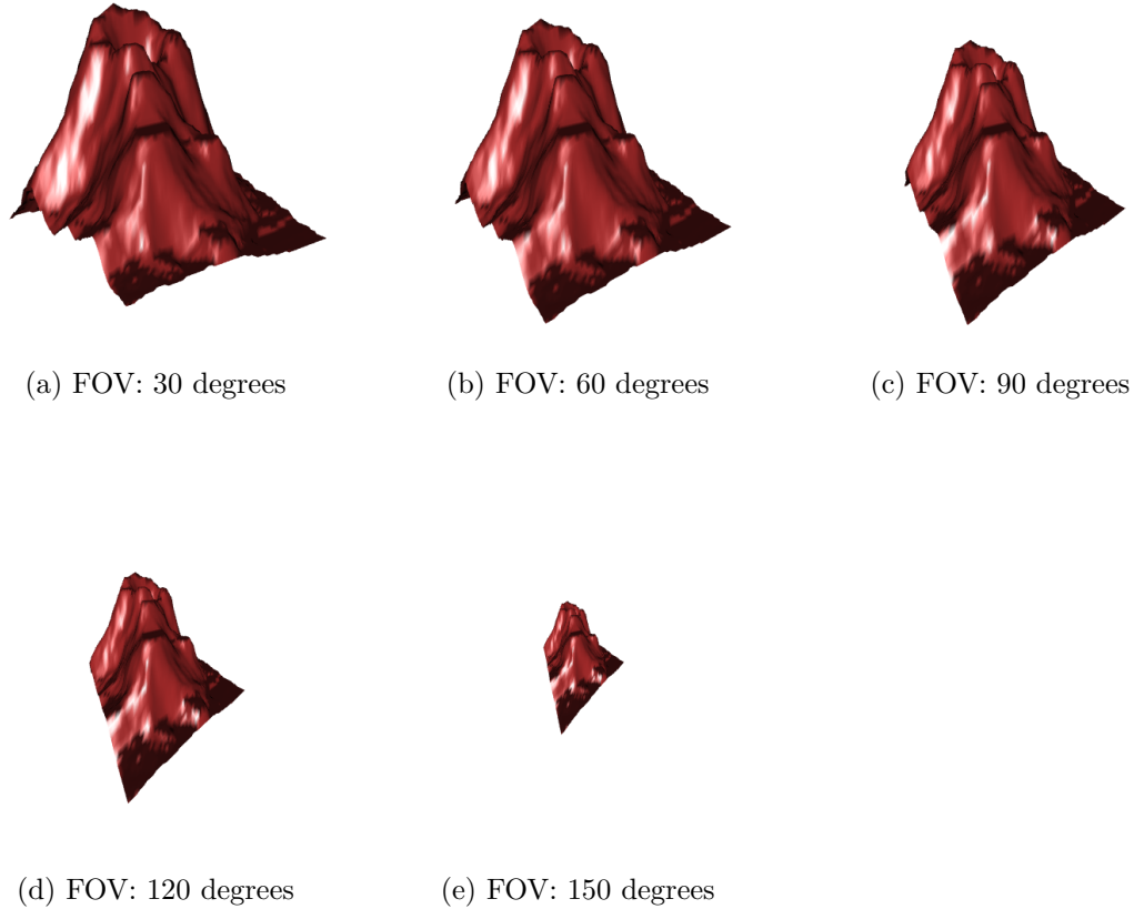
Figure 2.6: Multiple charts of the volcano dataset (R Core Team 2024) rendered using the rgl package (Murdoch and Adler 2023) in R. Each chart has a different field-of-view parameter, with the amount of distortion increasing as the field-of-view (FOV) increases.
