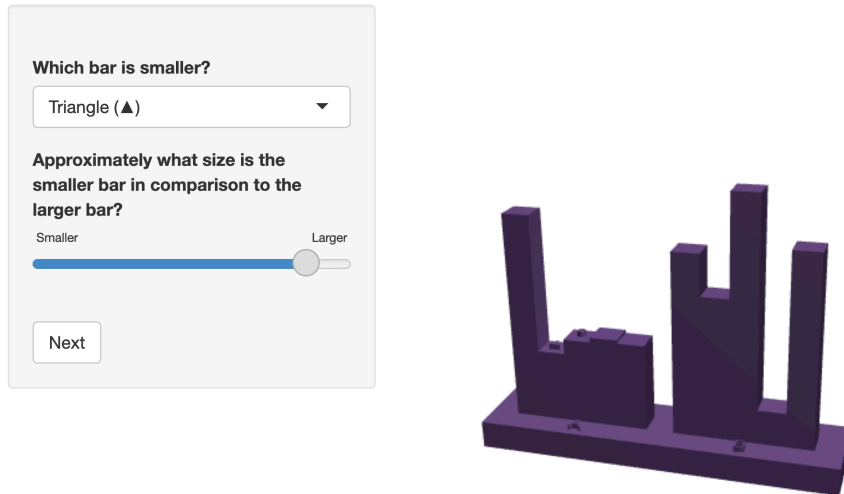
Figure 3.10: Screenshot of the applet collecting data for a 3D rendered chart task. Participants were asked to select which bar (circle or triangle) was smaller, and then to estimate the ratio of the smaller bar to the larger bar.
