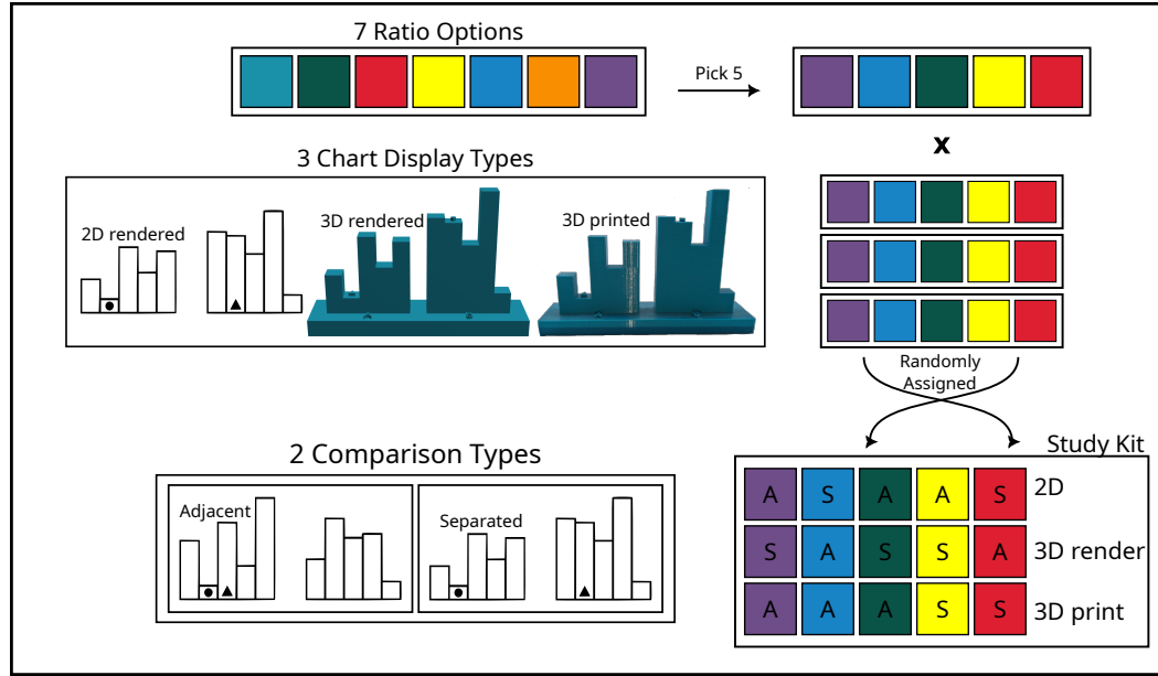
Figure 3.7: A graphical representation of the study design. Only five of the seven ratios were used in each kit; at least one of the smallest or largest ratios were included along with 4 other charts; each selected ratio was displayed in all 3 mediums. For each medium \times ratio combination, the comparison type (separated or adjacent) was randomly determined. A total of 21 kits of 3D printed charts were created to include all combinations of the five ratios.
