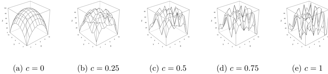
Figure 5.2: Mixture distribution of Equation 5.1 using the formula for the top half of a sphere. As c approaches 1, the distribution resembles uniform random noise.
