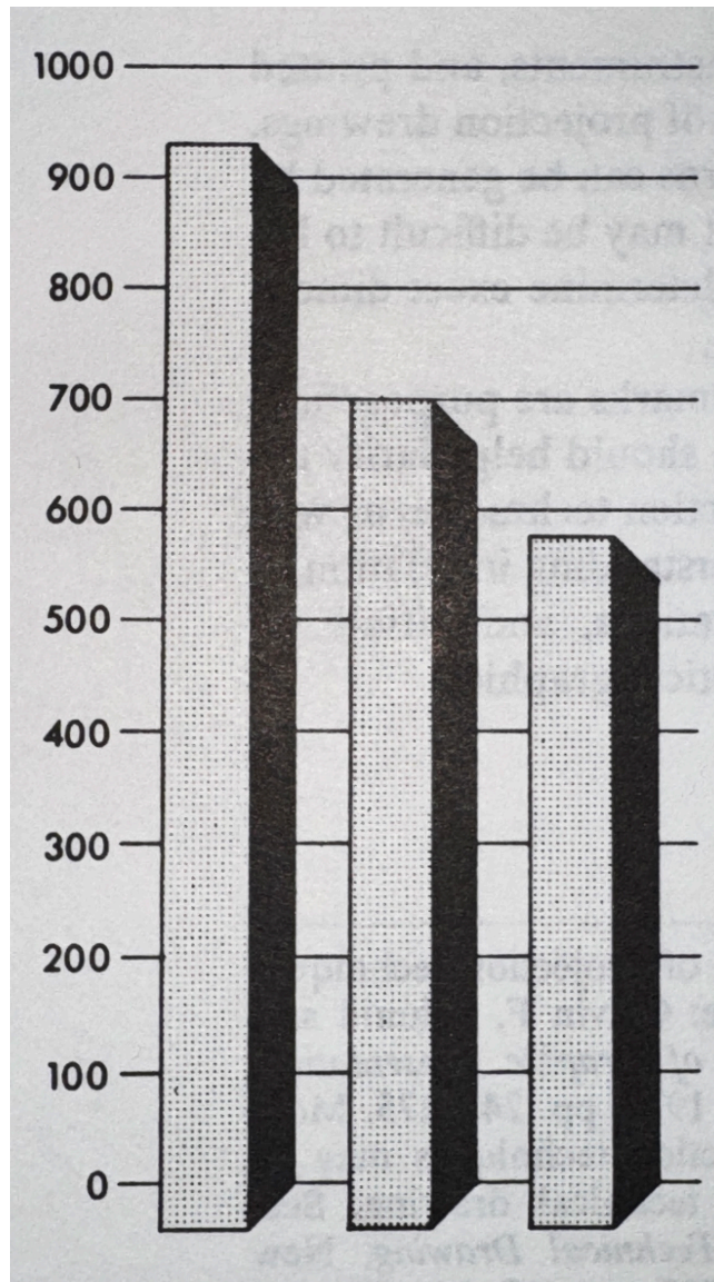
Figure 2.5: Figure in Statistical Graphics: Design Principles and Practices. The viewing angle for this chart would have viewers overestimate the values of the bars
