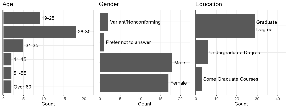
Figure 3.8: Demographic characteristics of participants in the study.
