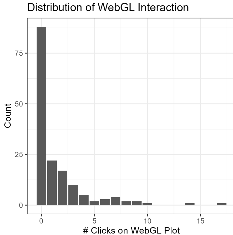
Figure 3.13: Participant clicks on the WebGL interface (left) in order to interact with the plot. Most participants did not interact with the WebGL interface, perhaps because they did not realize that interacting was an option, but some participants utilized the interactivity heavily. (Right) Participant interactivity was not associated with increased accuracy.
