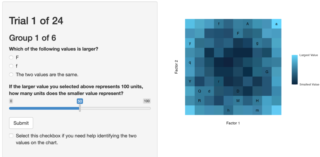
Figure 5.6: Graphics experiment page. Each trial contained two questions about a pair of stimuli, and a check box that displays the location of the stimuli if needed.
