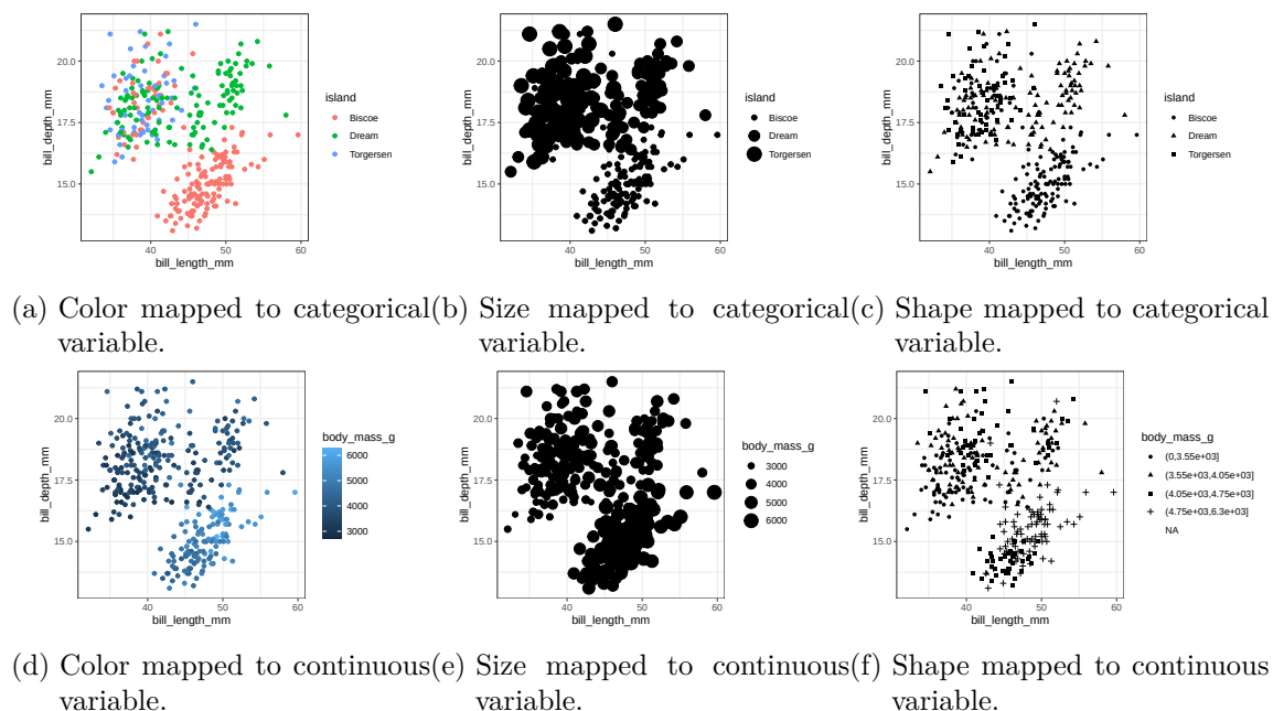
Figure 2.8: Examples of color, size, and shape for scatterplots of the penguins dataset (Horst, Hill, and Gorman 2020).
