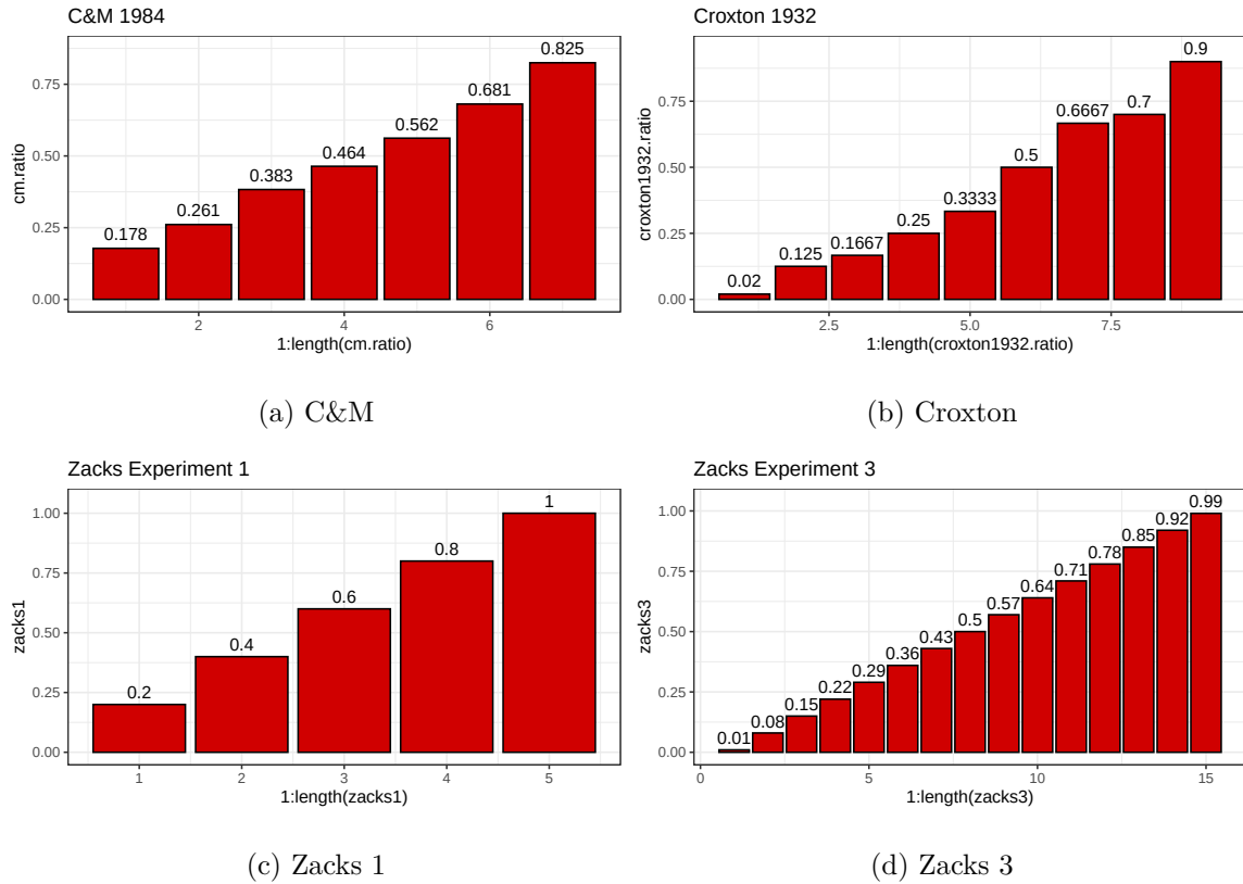
Figure 2.11: Ratios used by several studies
