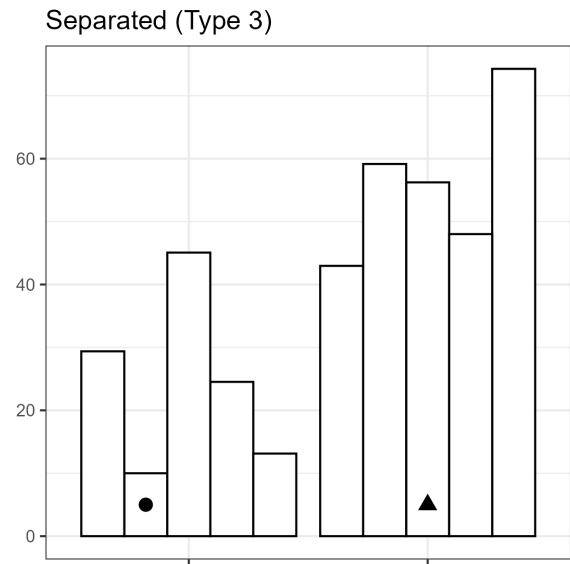
Figure 3.2: Cleveland and McGill (1984b) used two different types of grouped bar charts: comparisons between adjacent bars, and comparisons between separated bars. It is widely acknowledged that comparisons between separated bars (Type 3 comparisons, in Cleveland & McGill's terminology) are more difficult and error-prone.
