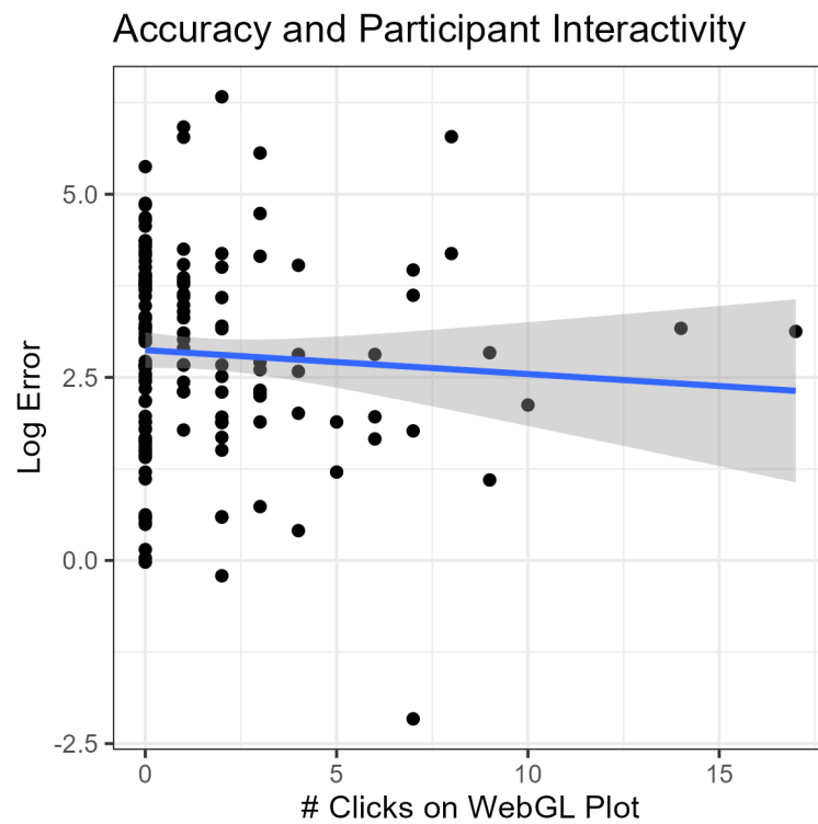
Figure 3.14: Participant clicks on the WebGL interface (left) in order to interact with the plot. Most participants did not interact with the WebGL interface, perhaps because they did not realize that interacting was an option, but some participants utilized the interactivity heavily. (Right) Participant interactivity was not associated with increased accuracy.
