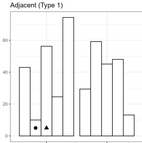
Figure 3.1: Cleveland and McGill (1984b) used two different types of grouped bar charts: comparisons between adjacent bars, and comparisons between separated bars. It is widely acknowledged that comparisons between separated bars (Type 3 comparisons, in Cleveland & McGill's terminology) are more difficult and error-prone.
