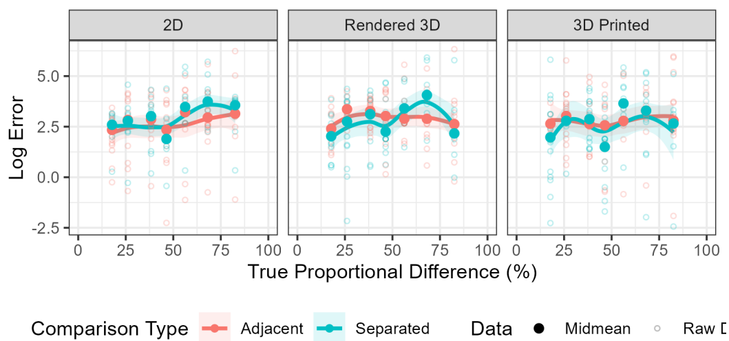
Figure 3.11: Midmeans and observed values of log absolute errors for the true ratio of bars. Summary lines are computed from raw data using a loess smooth.
