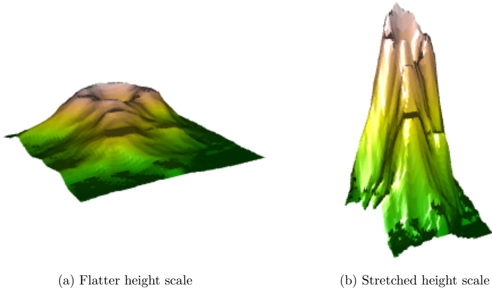
Figure 2.10: Two figures representing the volcano dataset (R Core Team 2024) using different height scaling factors. Both figures use the same color scale, but there is no “correct” translation of color into the measurable height.
