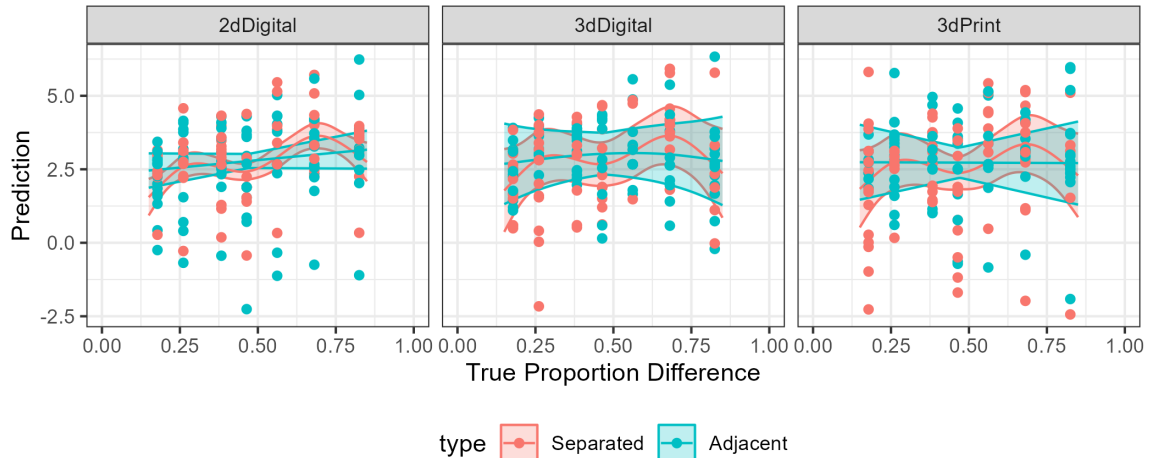
Figure 3.12: Predictions with standard errors for fixed effects in a generalized additive model with splines for ratio by comparison and ratio by display method. It is clear that the separated comparisons are easier to estimate when small, right around 50%, or large, and harder to estimate between these points. What is interesting is that no such trend is present for adjacent comparisons.
