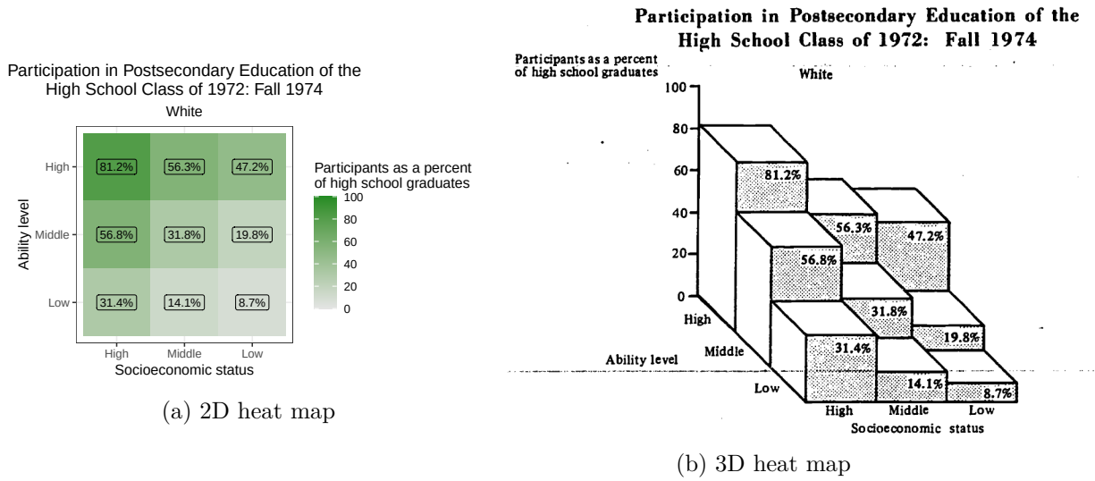
Figure 2.9: Heat maps created from with data from (XXX). The 2D heat map represents the percentage of high school graduates using a gradient color scale, whereas the 3D heat map uses height.
