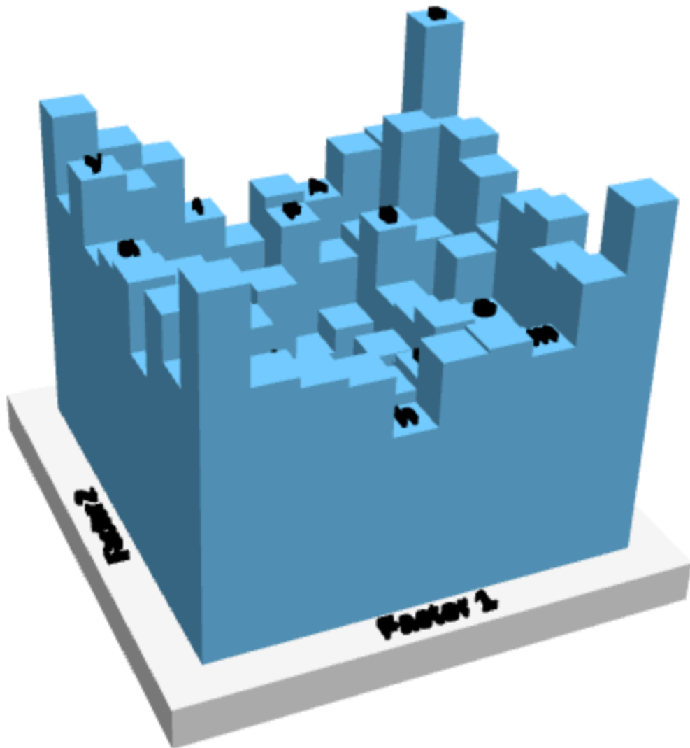
Figure 5.4: RGL rendering of Data Set 2 for 3dd charts.
