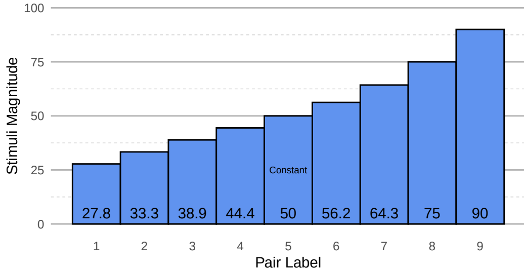
Figure 5.1: Values for stimuli in the heatmap experiment. All values are paired with the constant stimuli of 50 units, creating nine pairs of stimuli.
