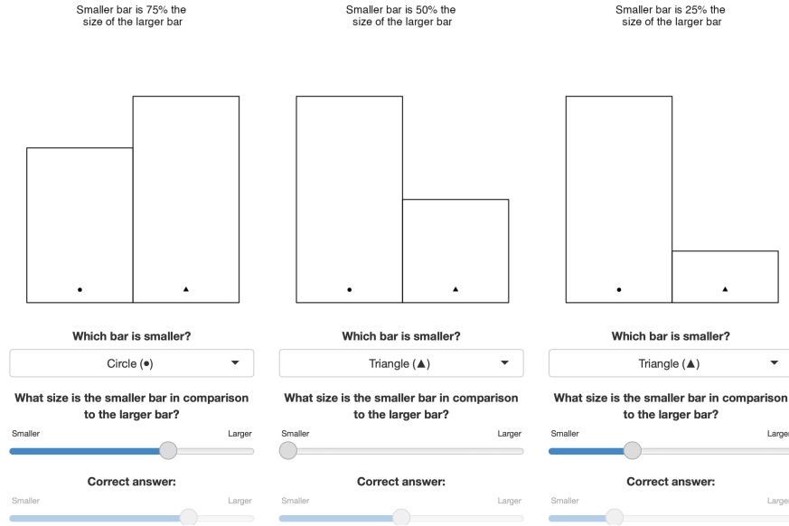
Figure 3.9: Screenshot of Shiny application practice screen. Three 2D bar charts with different ratios were provided, along with sliders indicating the correct proportion. Participants could practice with the sliders and preview the questions that would be asked as part of the task.
