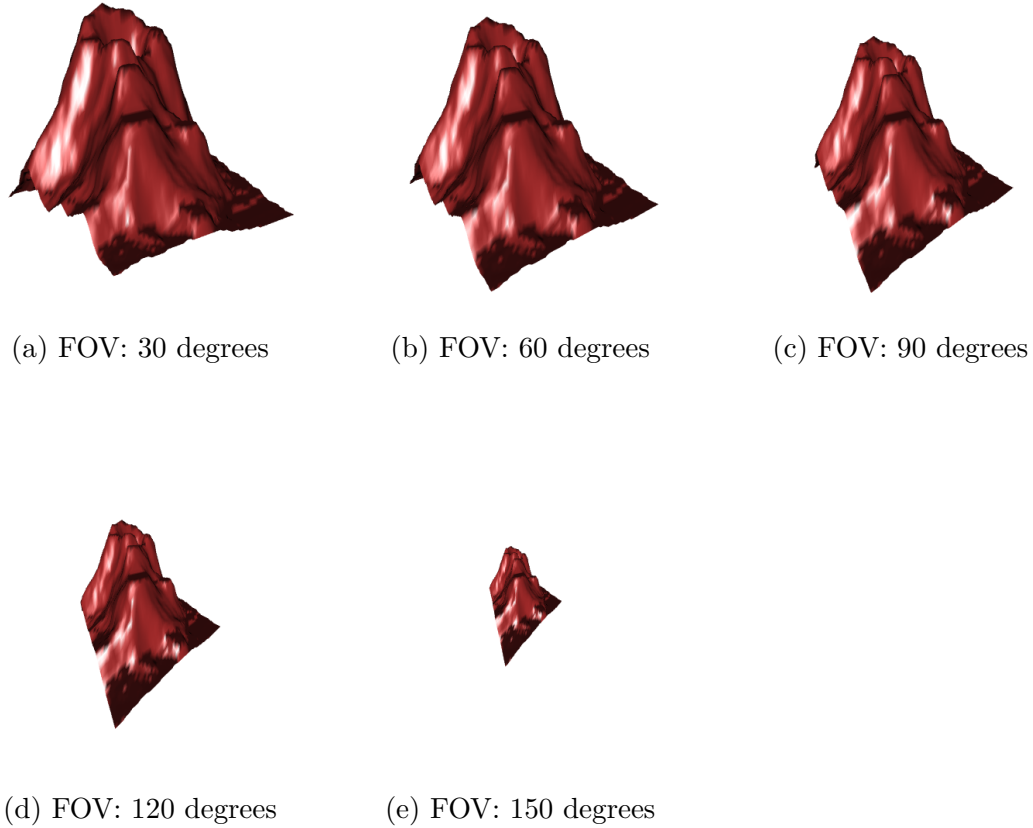
Figure 1.6: Multiple charts of the volcano dataset (R Core Team, 2024) rendered using the rgl package (Murdoch & Adler, 2023) in R. Each chart has a different field-of-view parameter, with the amount of distortion increasing as the field-of-view (FOV) increases.
