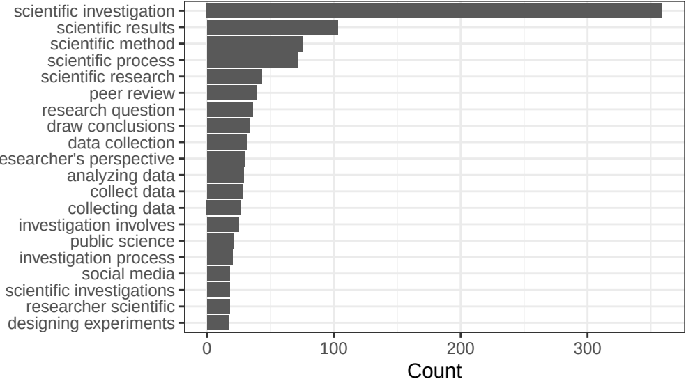
Bigram
