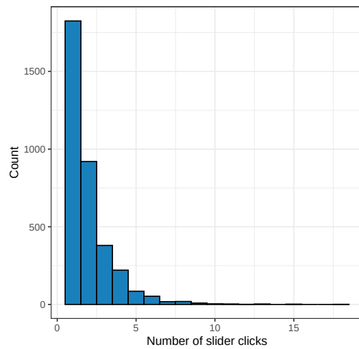
(a) Histogram
