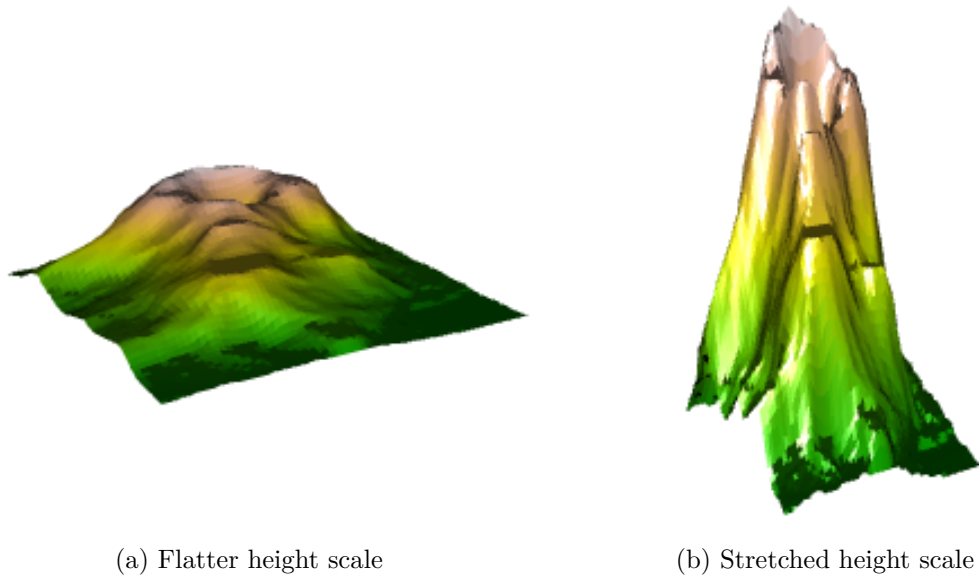
Figure 2.10: Two figures representing the volcano dataset [volcano] using different height scaling factors. Both figures use the same color scale, but there is no “correct” translation of color into the measurable height.
