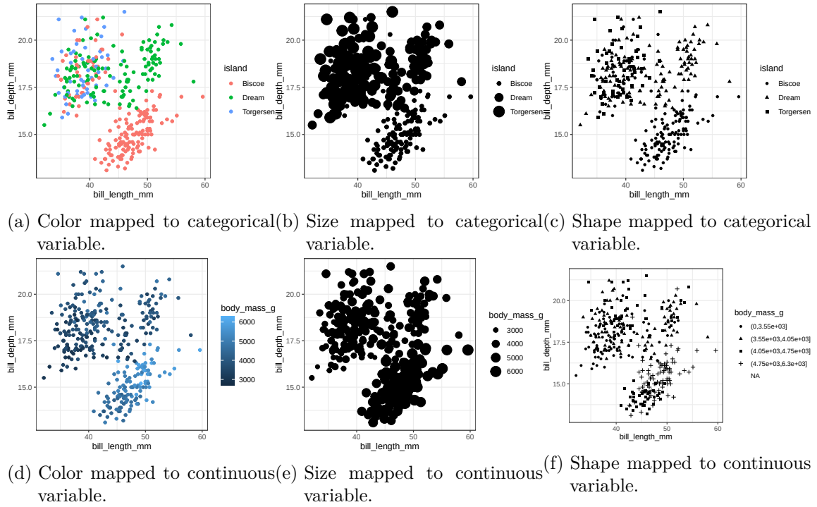
Figure 2.11: Examples of color, size, and shape for scatterplots of the penguins dataset (Horst, Hill, and Gorman 2020).
