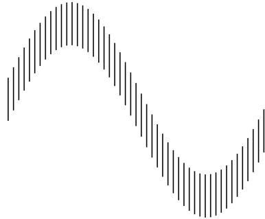
(a) Sine Illusion
