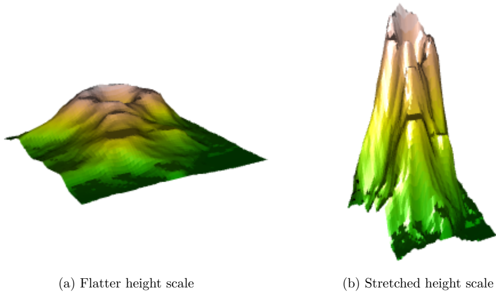
Figure 2.7: Two figures representing the volcano dataset [volcano] using different height scaling factors. Both figures use the same color scale, but there is no “correct” translation of color into the measurable height.
