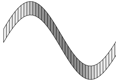
(b) 3D surface with similar features
