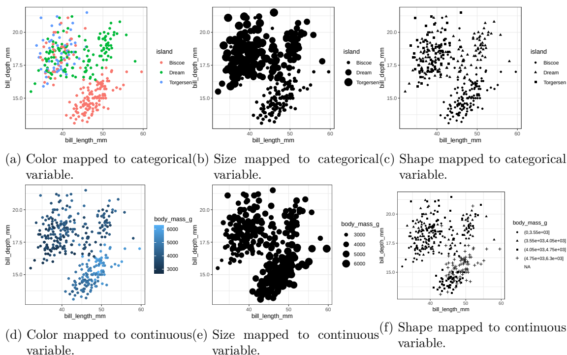
Figure 2.5: Examples of color, size, and shape for scatterplots of the penguins dataset [pen-guins].
