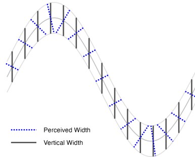
(c) Perceived vs. actual length
