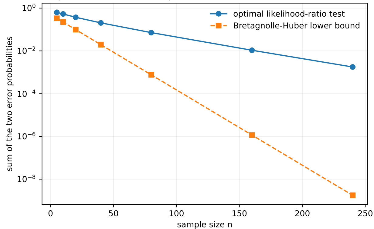
Nearby models cannot be separated faster than their information allows
