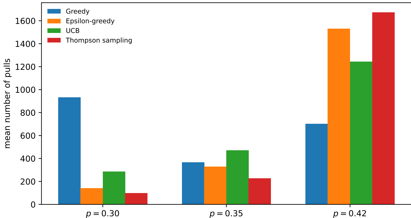
Where each algorithm spends its samples
