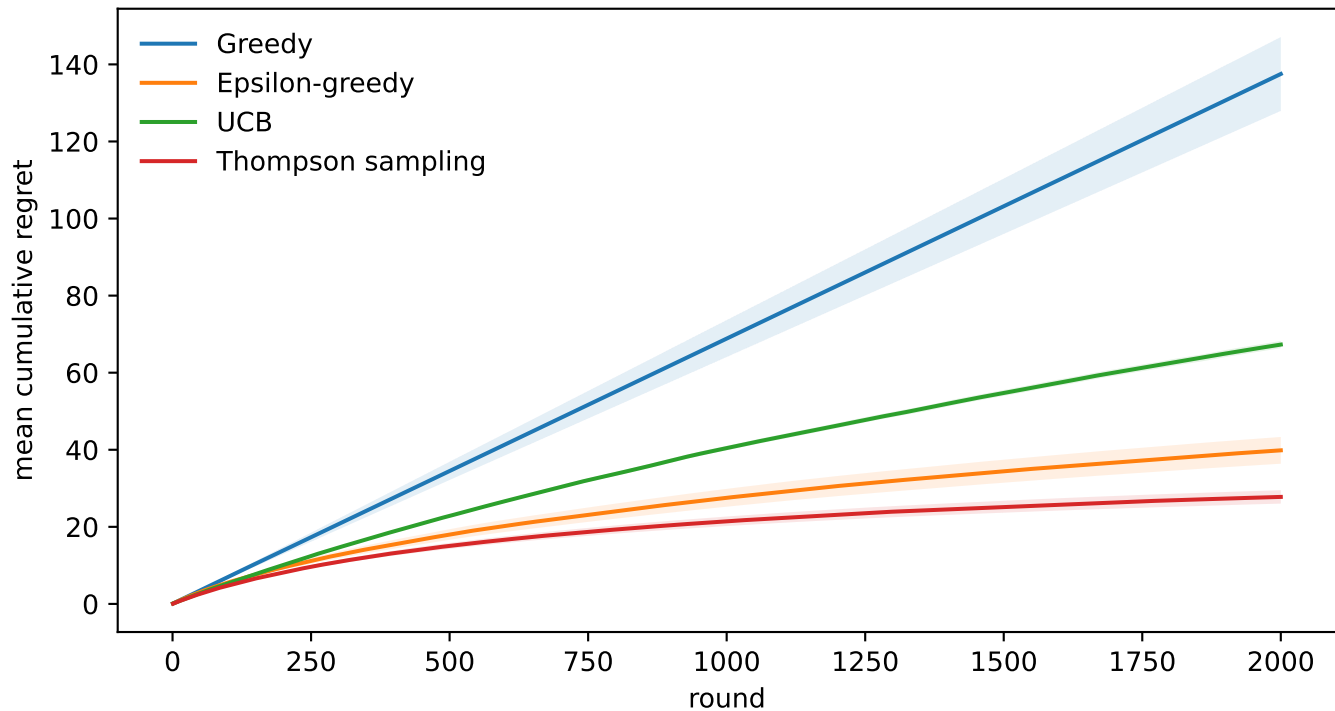
Regret in a three-arm Bernoulli bandit
