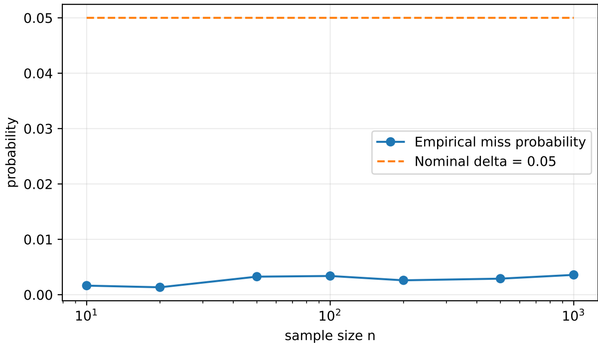
Fixed-time Hoeffding intervals are conservative
