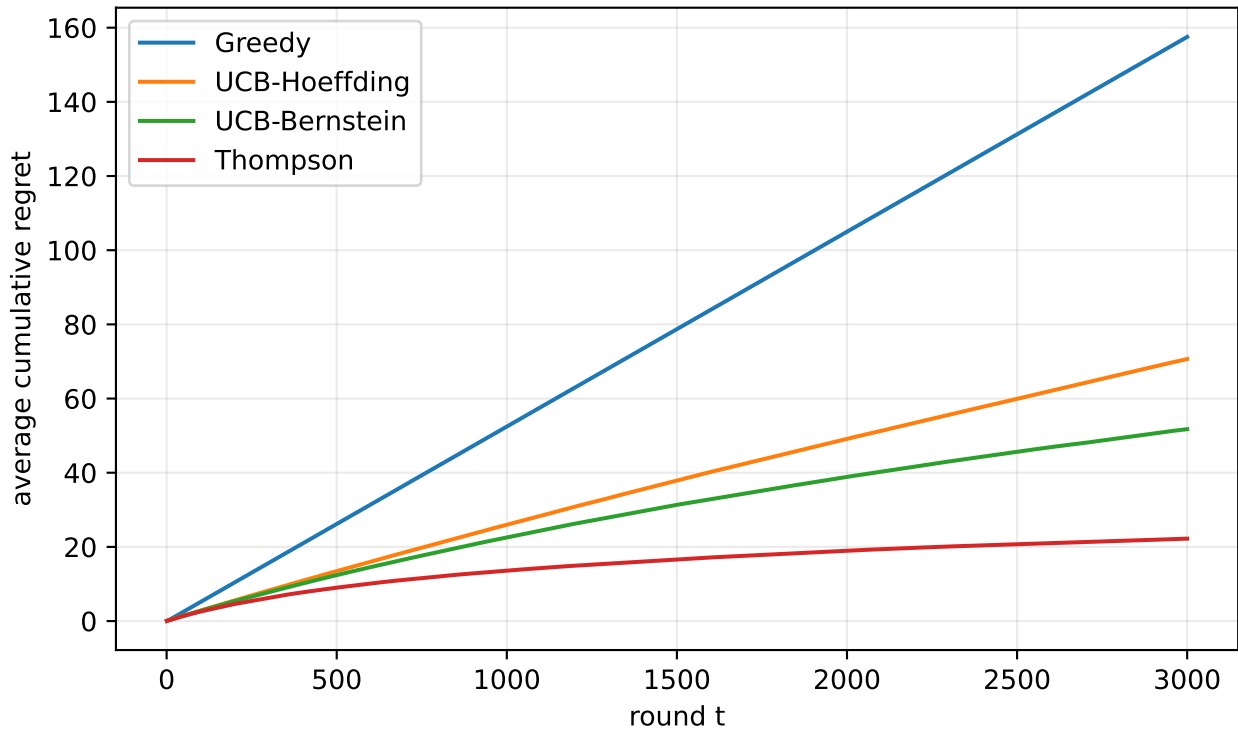
Concentration turns uncertainty into action
