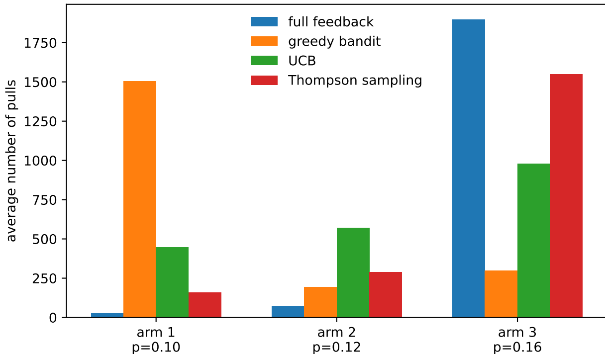
Which arms did the algorithms actually try?
