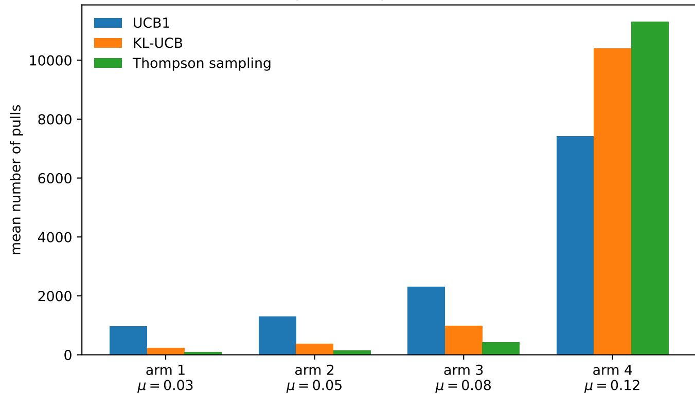
Where the algorithms spent 12,000 observations
