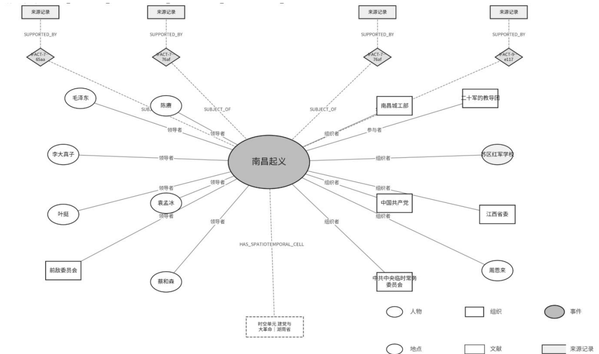
图 6 “南昌起义”事件中心时空知识子图示例；English: Figure 6 Event-centered spatiotemporal subgraph of the Nanchang Uprising
