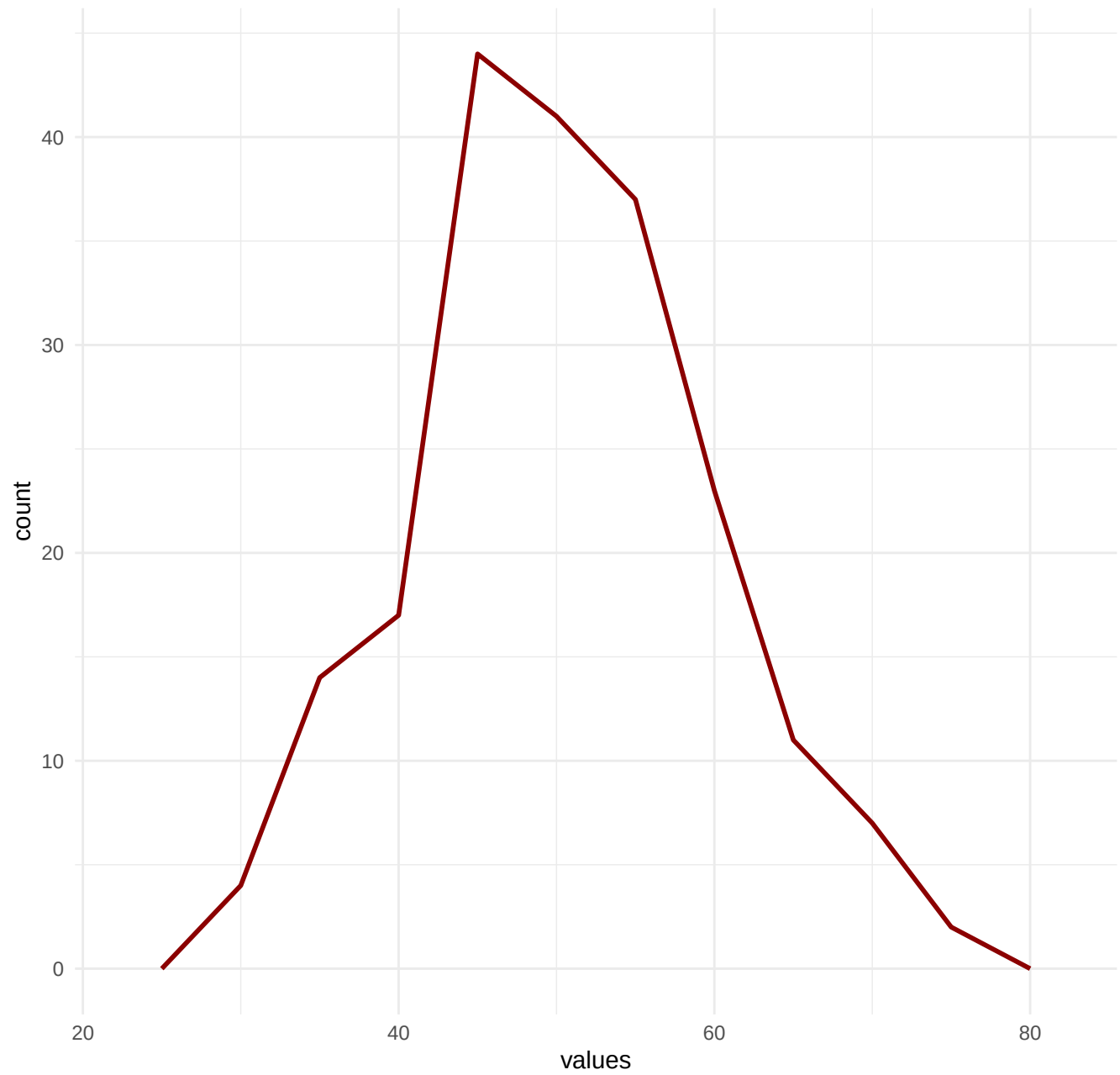
Frequency Polygon
