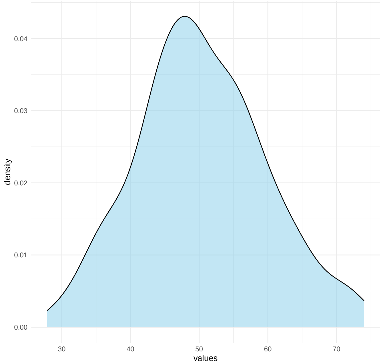
Density Plot
